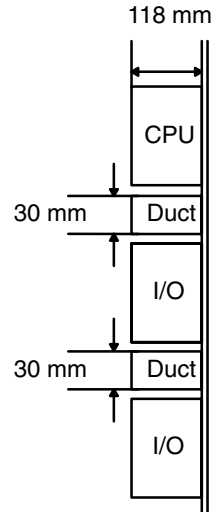
C200HS-CPU01-E/CPU01-EC/CPU03-E
