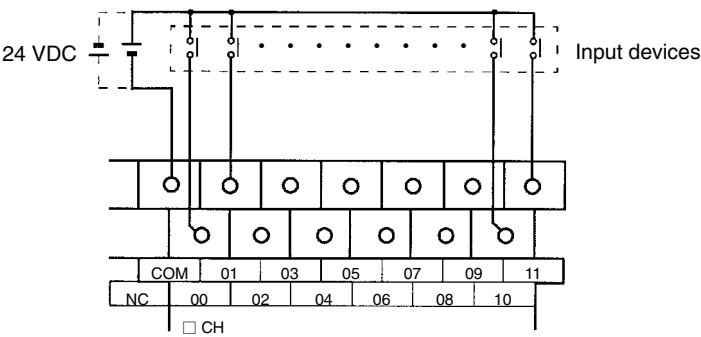
CPM1A-20EDR/20EDR1/EDT/EDT1
