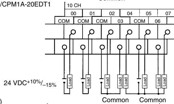
CPM1A-30CDT1-□(-V1)
