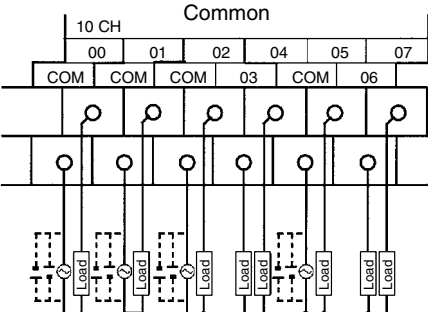
CPM1A-20CDR-□(-V1)/CPM1A-20EDR/20EDR1
