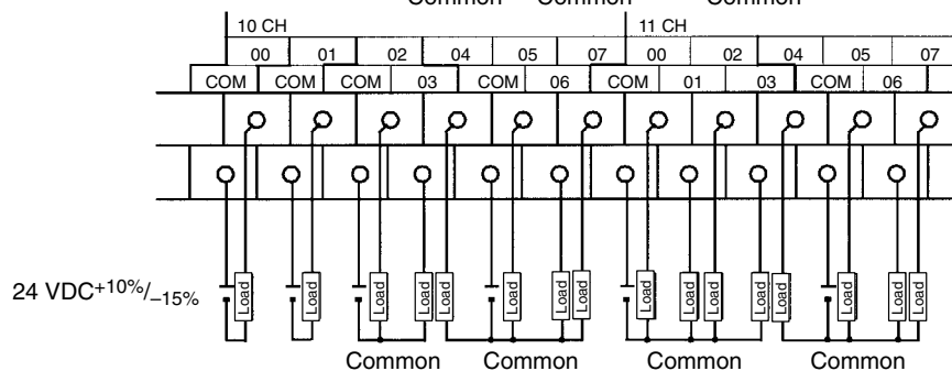
CPM1A-40CDT1-□(-V1)
