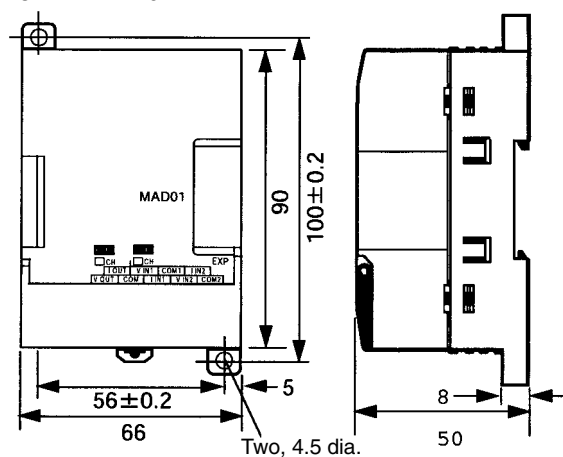
CPM1A-MAD01
