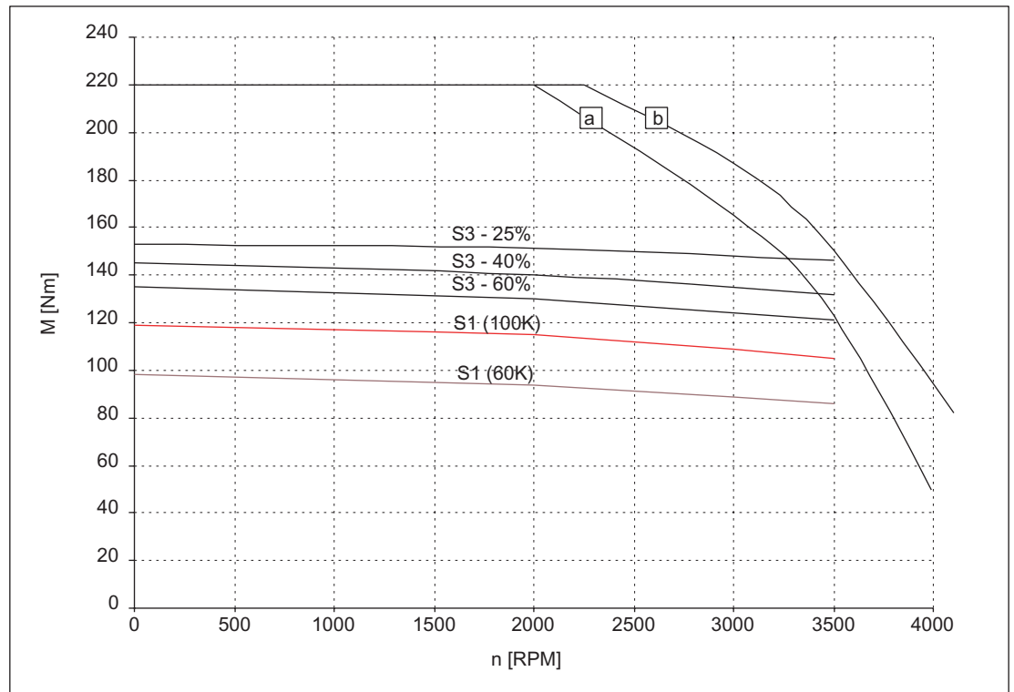
Figure 3-94 Speed-torque diagram 1FT6108-8WF7□
