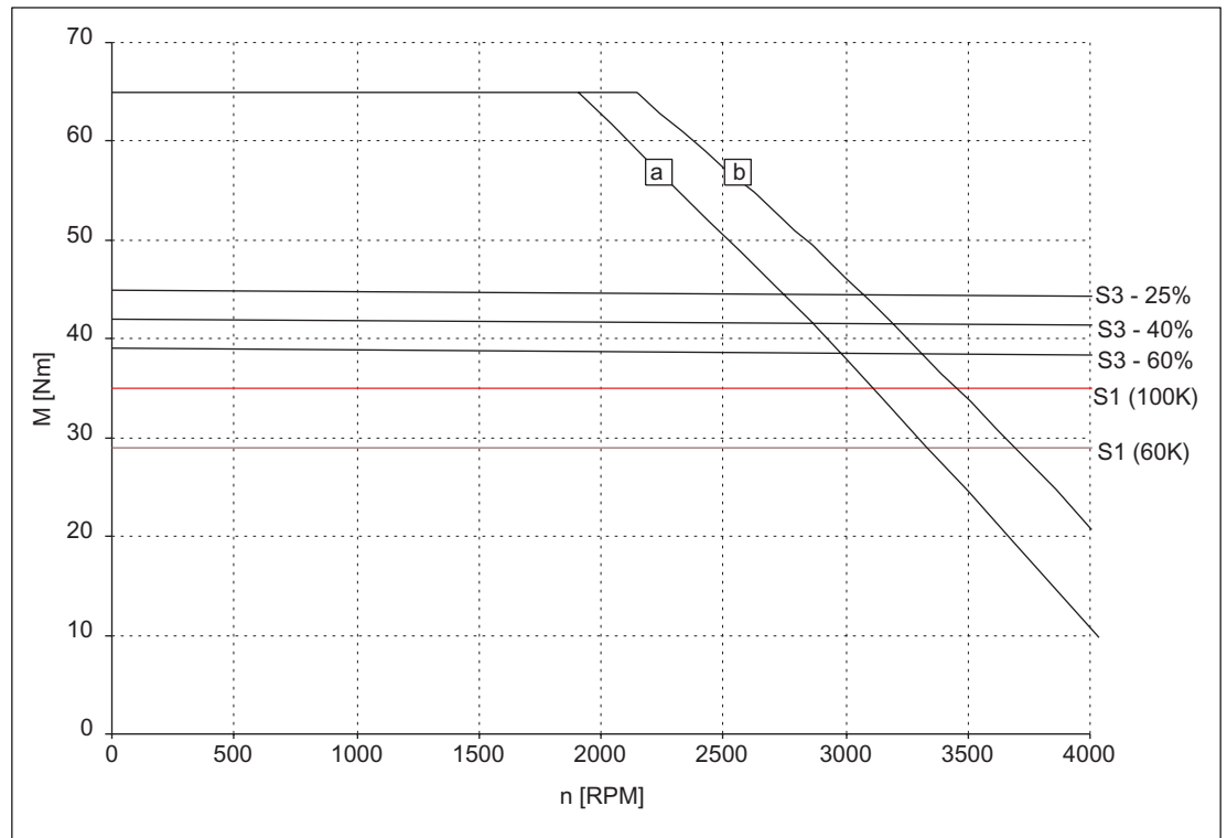
Figure 3-84 Speed-torque diagram 1FT6084-8WF7□
