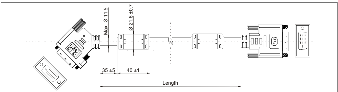
Figure 112: 5CASDL.0xxx-01 - Dimensions
