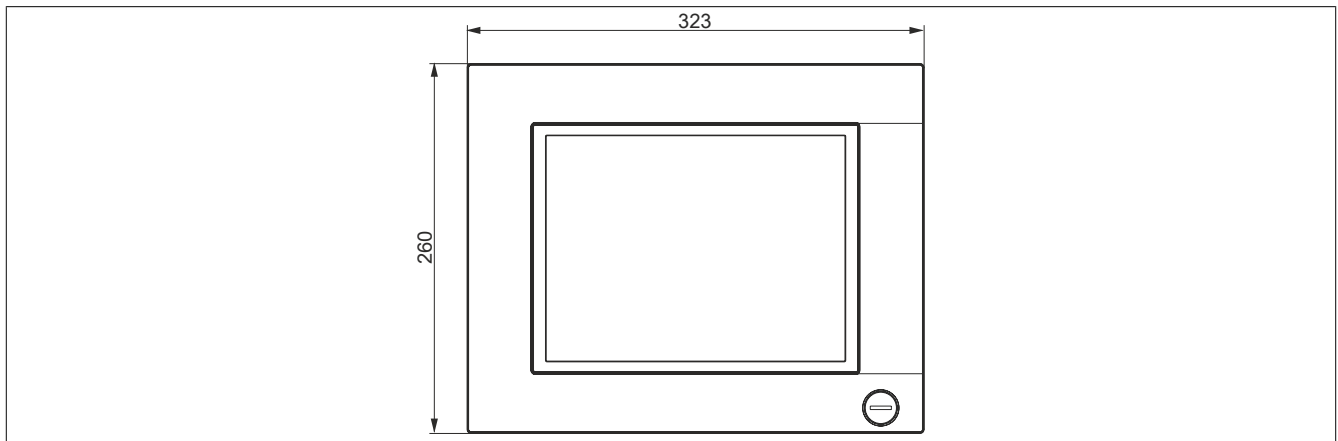
Figure 55: 5AP1120.1043-000 - Dimensions
