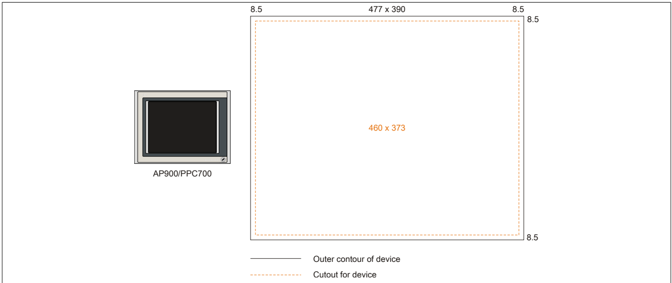
Figure 38: Mounting compatibility - 17" device - Horizontal1
