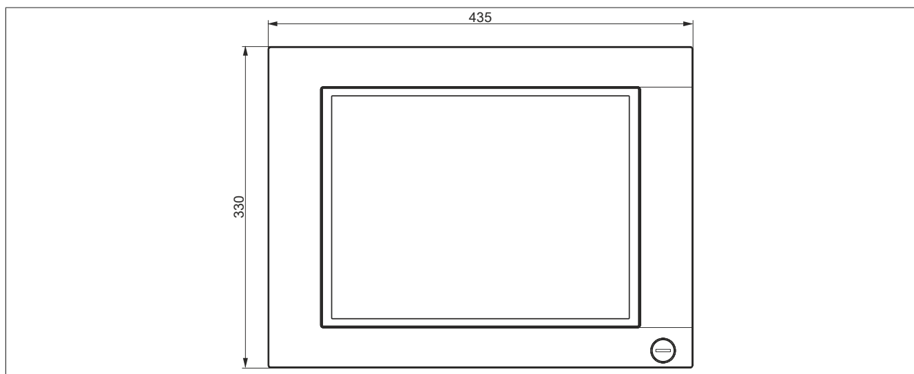
Figure 69: 5AP1120.1505-000 - Dimensions
