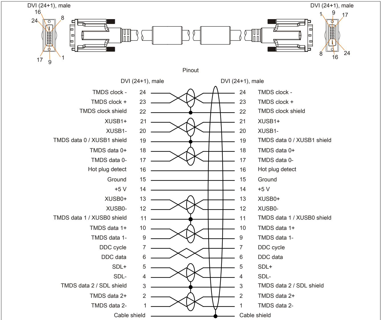
Figure 117: 5CASDL.0xxx-03 - Pinout
