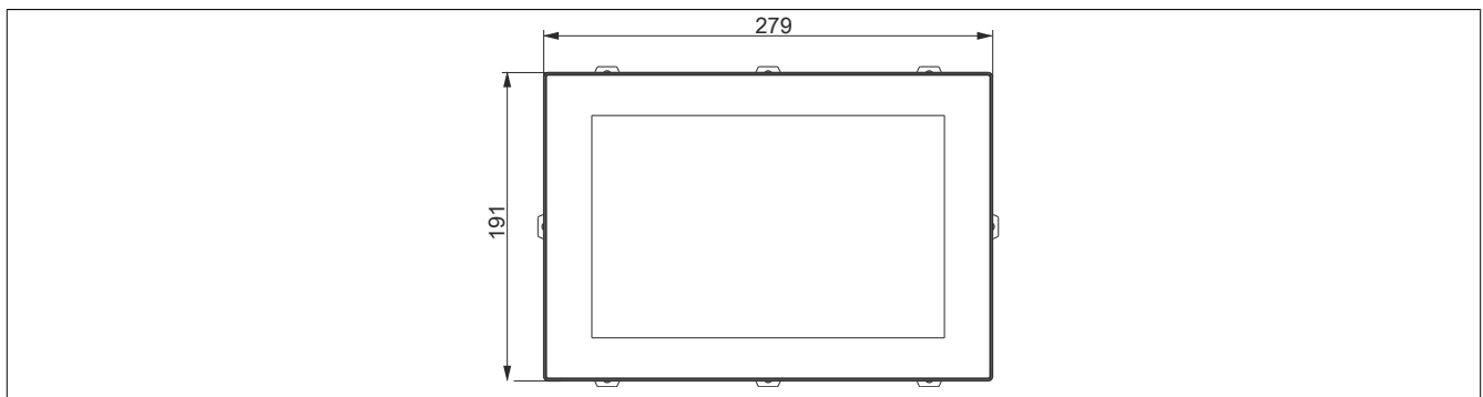
Figure 53: 5AP1130.101E-000 - Dimensions
