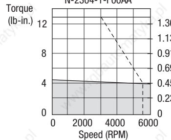
1398-DDM-010,-010x and N-2304-1-F00AA
