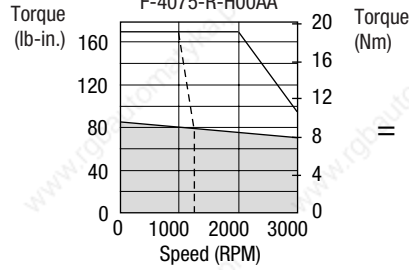
1398-DDM-075,-075x and F-4075-R-H00AA (3ø Input)
