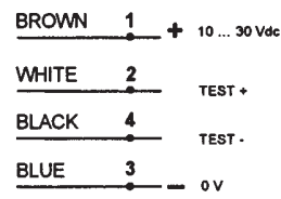
S5-5-G8/G12 (4 wires)
