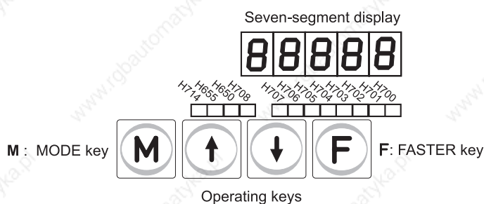
Illustration 25: Seven-segment display
