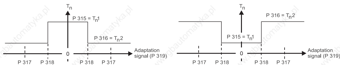
Illustration 70: T_n adaptation for the speed controller - Fig. 2
