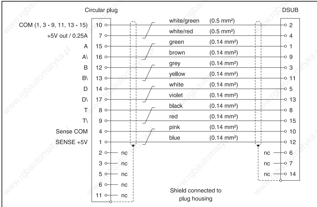
Figure 183: Cable schematic - 8BCE EnDat cable
