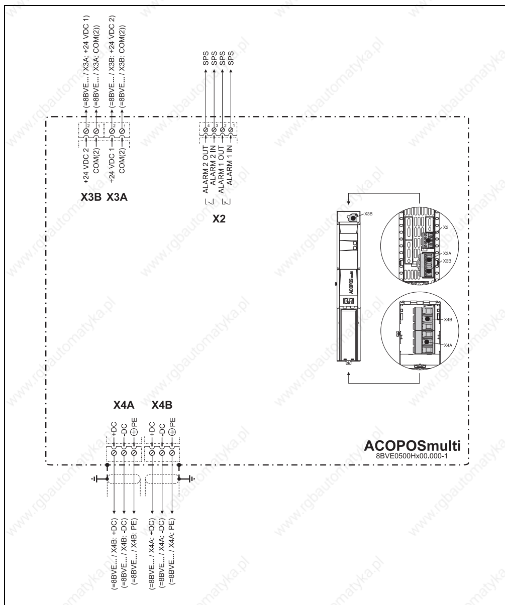
Figure 165: Overview of pin assignments - 8BVE0500Hx00.000-1
