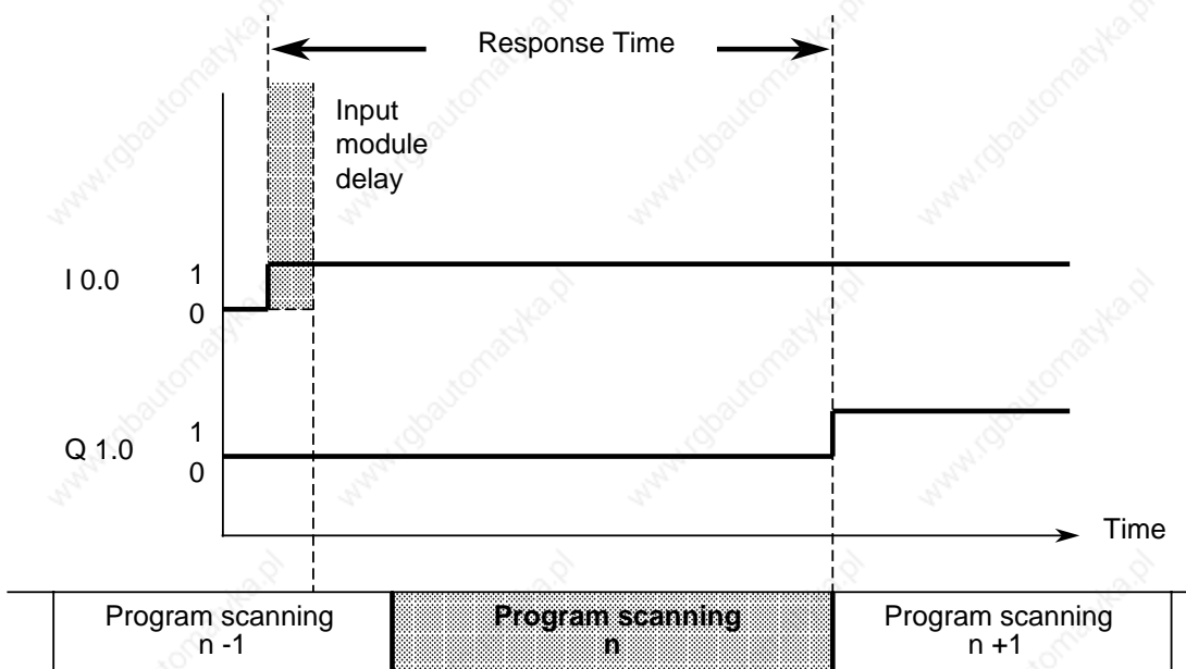
Figure 2-15. Response Time
