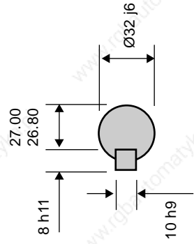
SHAFT DETAIL
