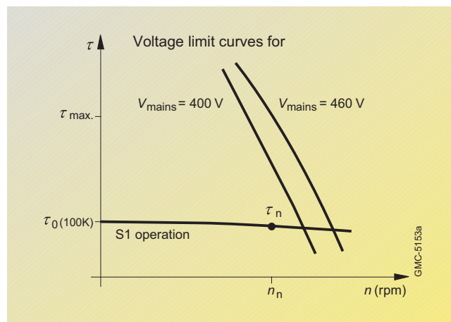
Fig. 2/6 Torque-speed characteristic
