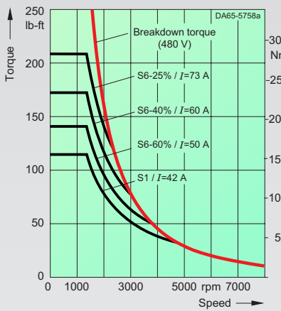
1PH7137-2.D...-.... max. breakdown torque: 347 lb-ft/471 Nm
