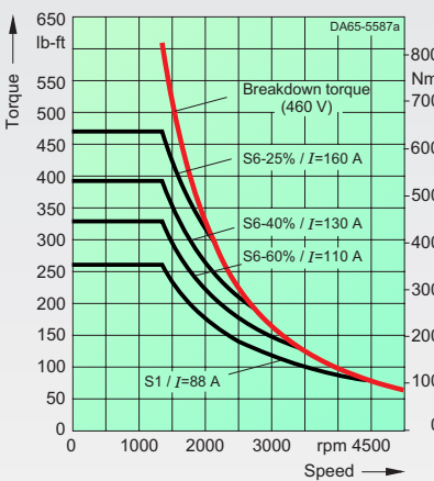
1PH7184-2.D...-.... max. breakdown torque: 607 lb-ft/823 Nm
