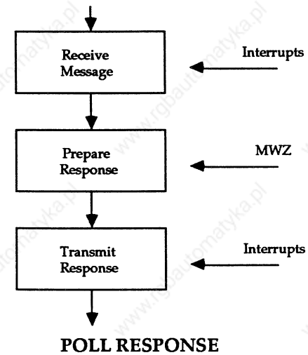
FIGURE 30 - ABC DATA EXCHANGE PROCEDURE DIAGRAMS
