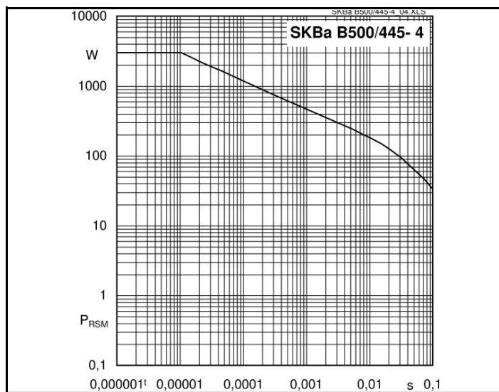
Fig. 7 Rated reverse power dissipation vs. time
