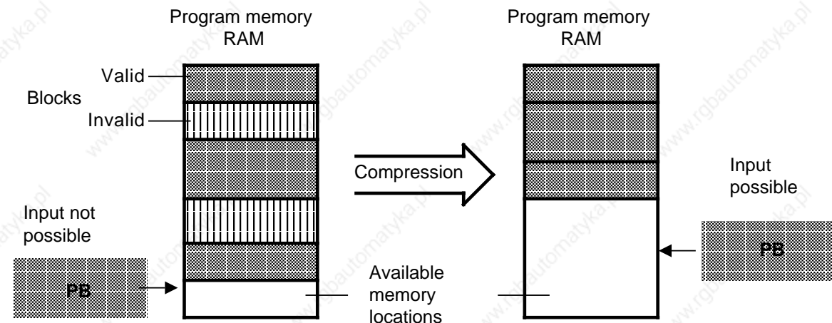
Figure 7-10. Compression Process
