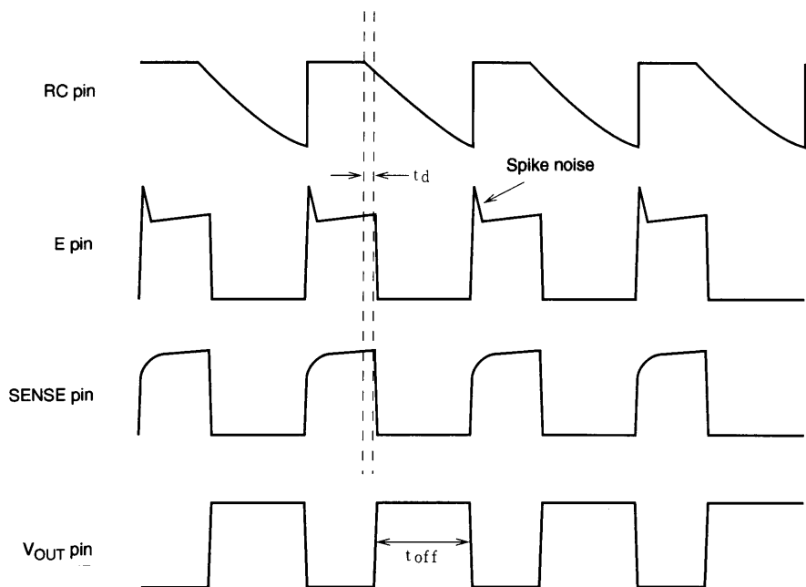
Figure 1 Switching Waveforms
