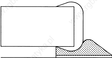
Poor wetting
