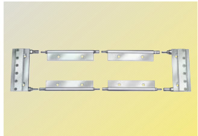
Fig. 4/14 Cooling profile with connector plugs (unconnected) and combination-distributor on each side. Total length <9.84 ft (3 m).
