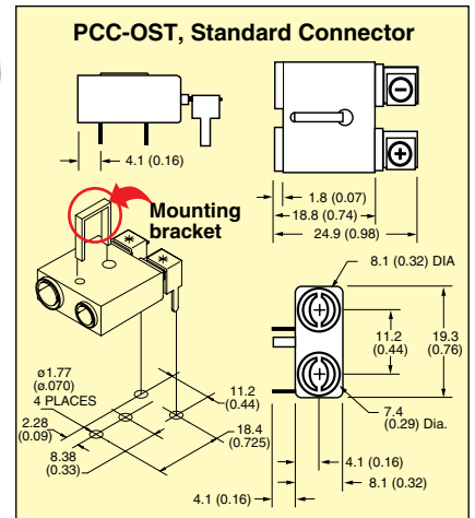
† A mounting bracket is supplied with each connector and must be used to securely mount the connector to the PC board.
