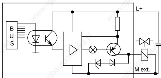
Simplified Schematic
