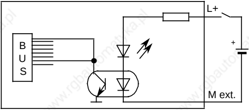
Block diagram
