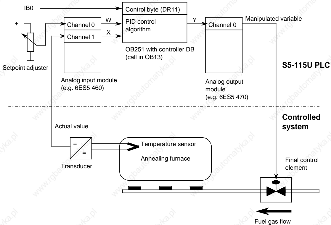
Figure 11-5. Process Schematic
