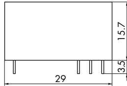
Hole diameter 1.3 mm
