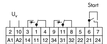
Switch-on wiper
