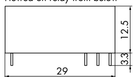
Hole diameter contacts 1.5 mm Hole diameter coil 1.3 mm
