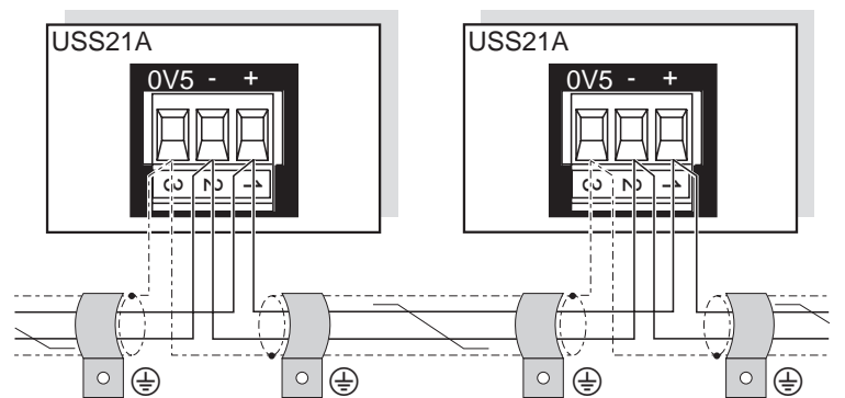
Fig. 22: RS-485 interface of the USS21A
