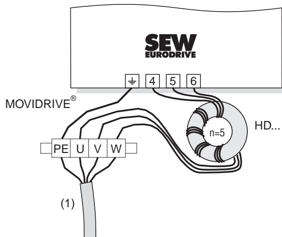
Fig. 13: Connecting HD... output chokes
