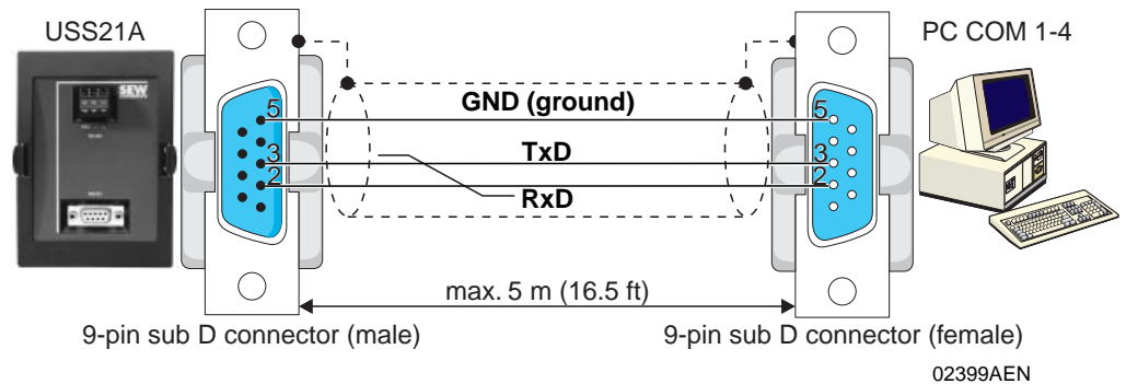
Fig. 21: Connection cable USS21A – PC
