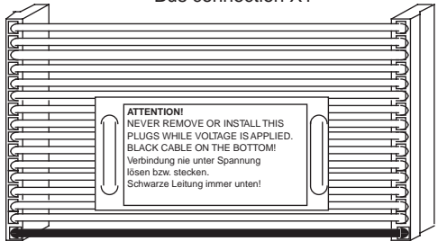
Programming Module MOD with Rating Plate
