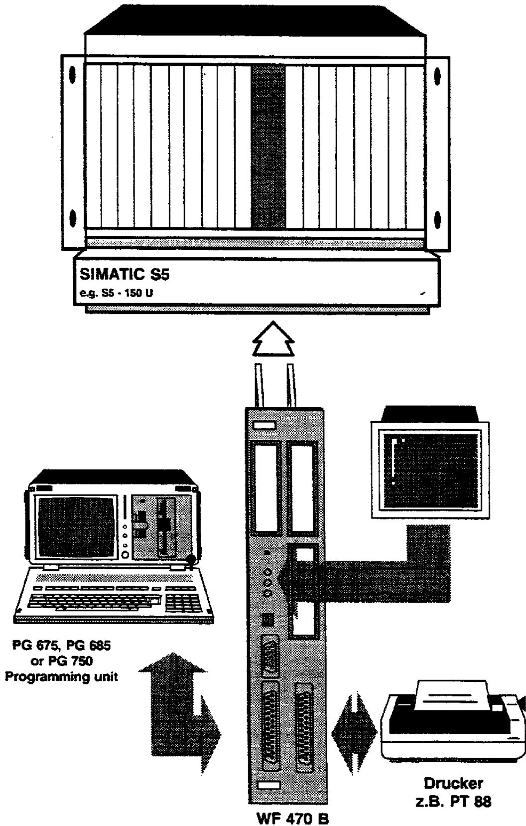
Fig. 2.3 Hardware configuration.
