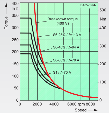
1PH7167-2.D... max. breakdown torque: 724 lb-ft/981 Nm
