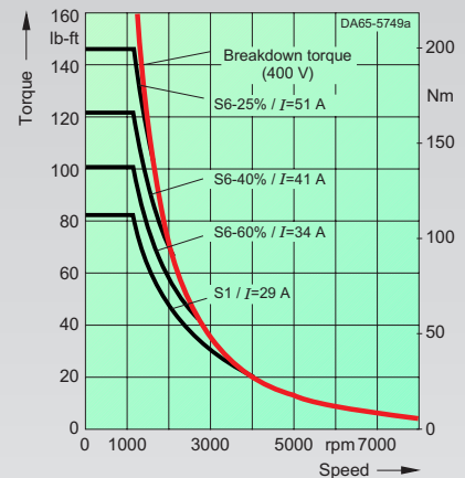
1PH7133-2.D... max. breakdown torque: 200 lb-ft/271 Nm
