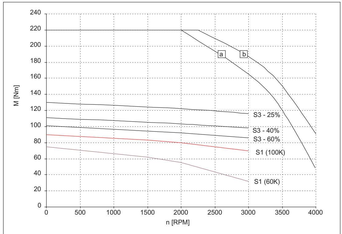
Figure 3-65 Speed-torque diagram 1FT6108-8SF7□
