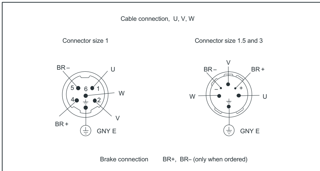
Figure 2-2 Power connection
