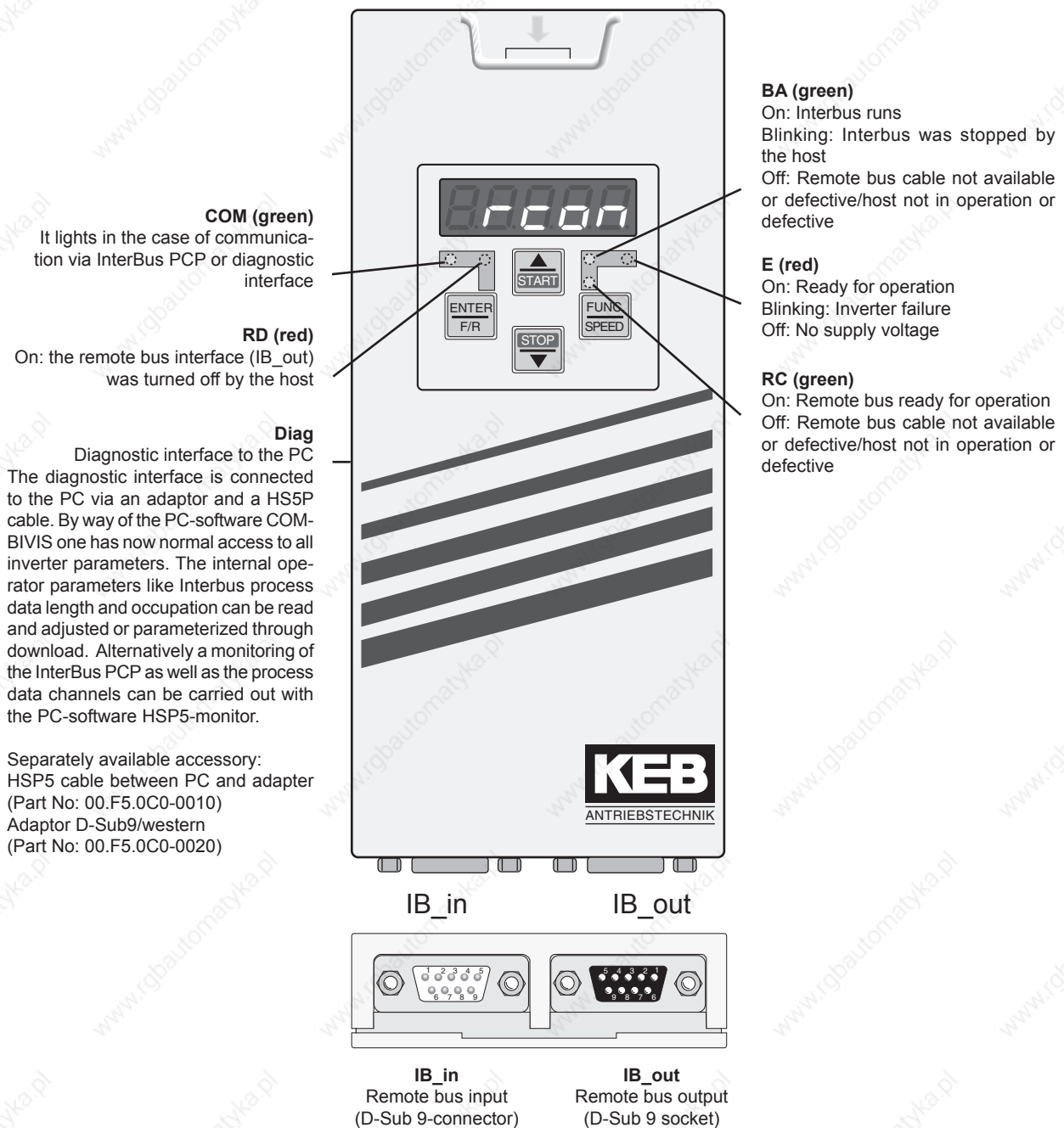
Fig. 11.1.6 InterBus operator
