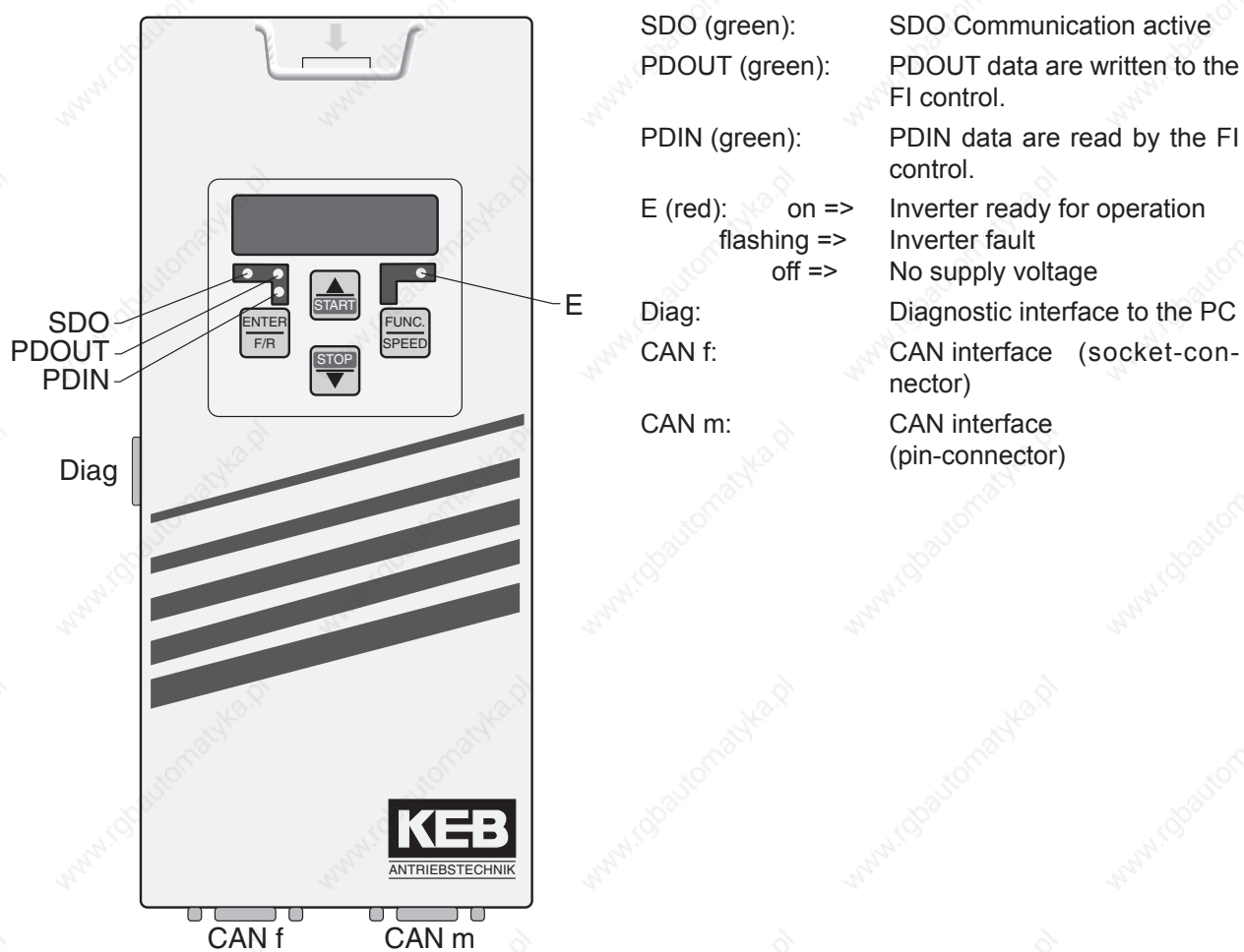
Fig. 11.1.7 CanOpen operator
