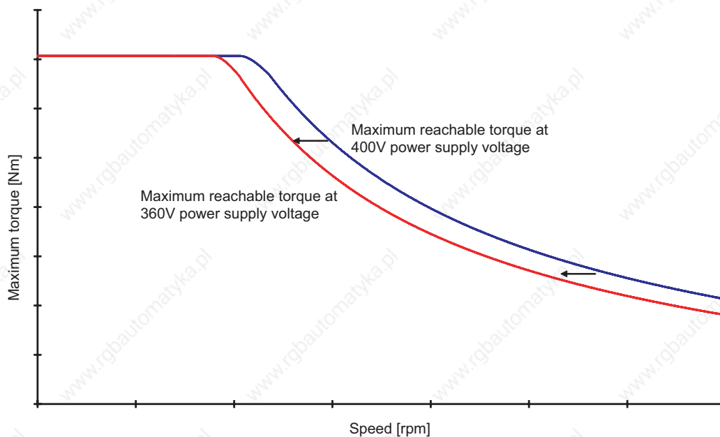
Figure 7.8.3.2.3 Shift of limiting characteristic
