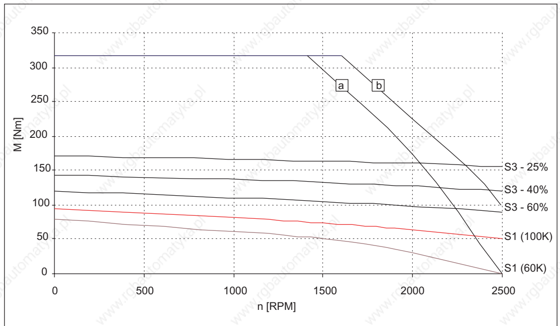
Figure 3-50 Speed-torque diagram 1FT6134-6AC71
