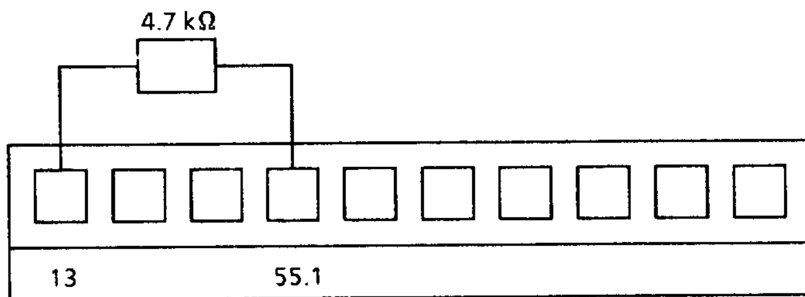
Fig. 3.10 Connector X1.1
