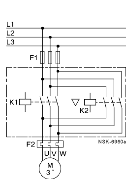
Power circuit
