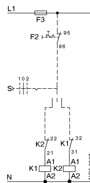
Control circuit for maintained-contact control
