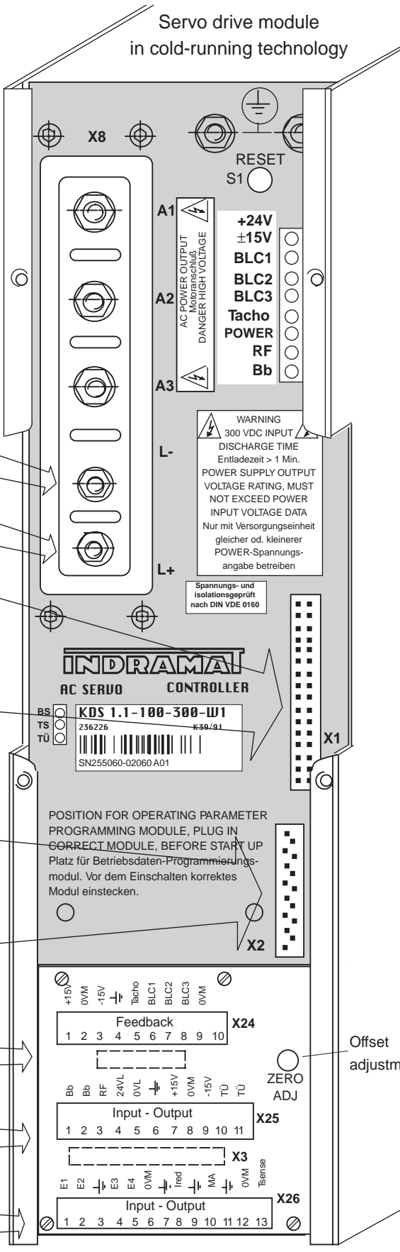
Figure 40: Front view of servo drive module KDS1 with accessories
