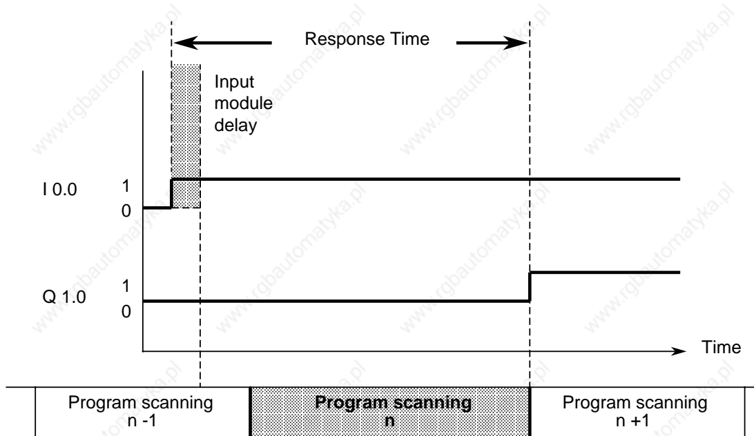
Figure 2-15. Response Time
