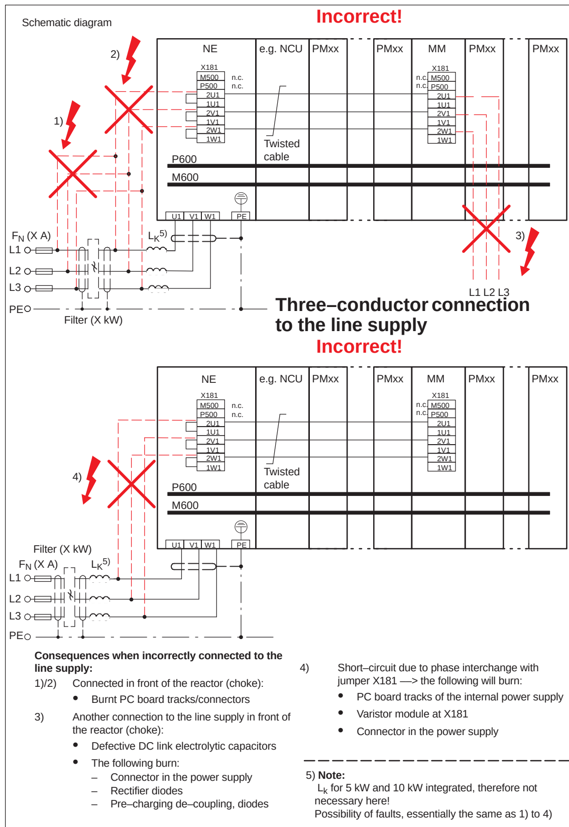
Fig. 8-31 Examples of three-conductor connection to the line supply that are absolutely prohibited
