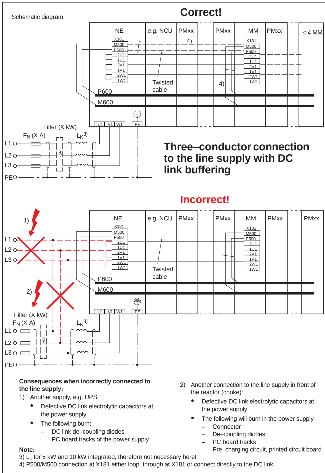
Fig. 8-32 Examples for correct and prohibited three-conductor connection to the line supply + DC link connection
