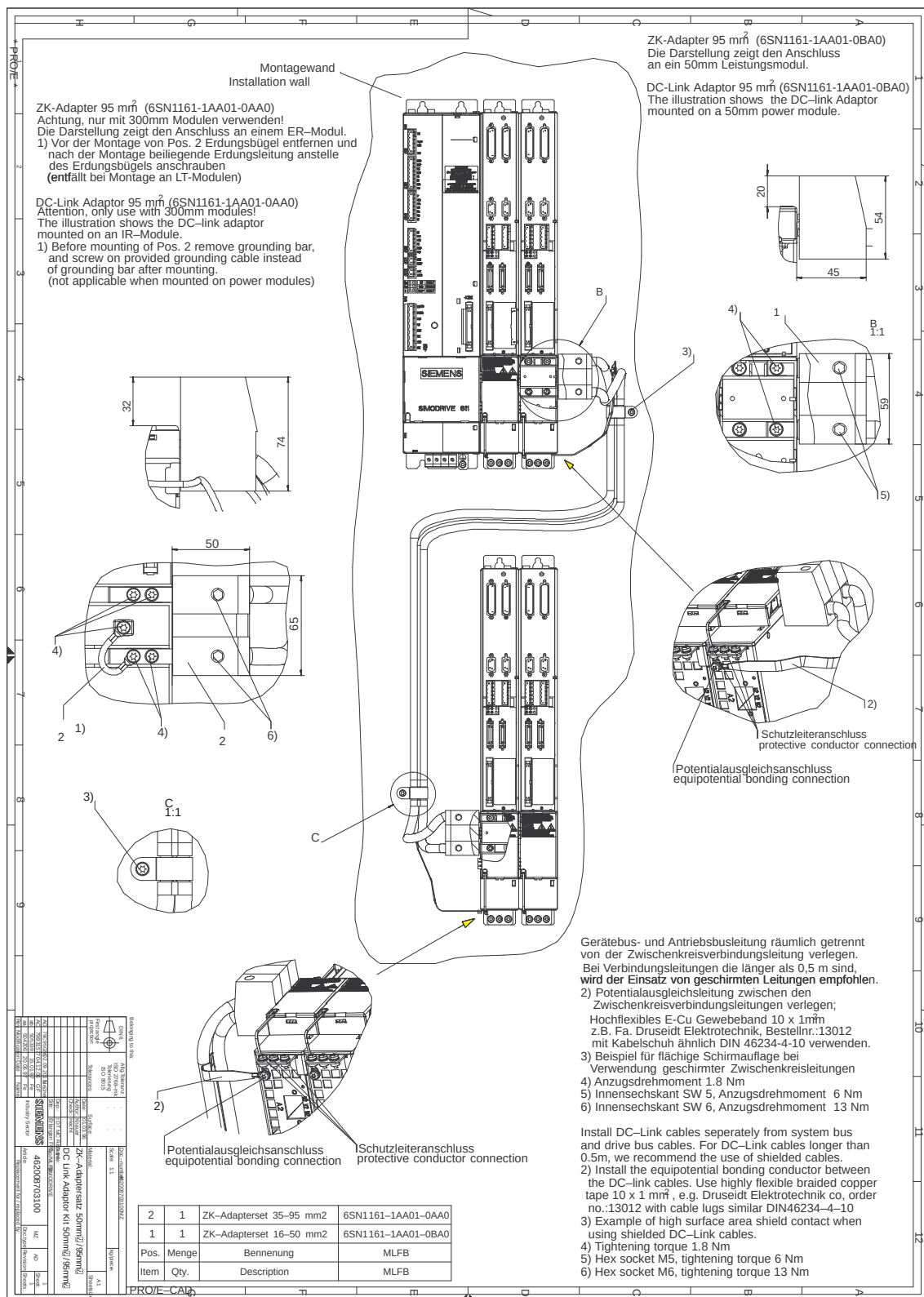
Fig. 12-60 DC link adapter set 16...50 mm² and 35...95 mm² 6SN1161-1AA01-0BA0/ -0AA0
