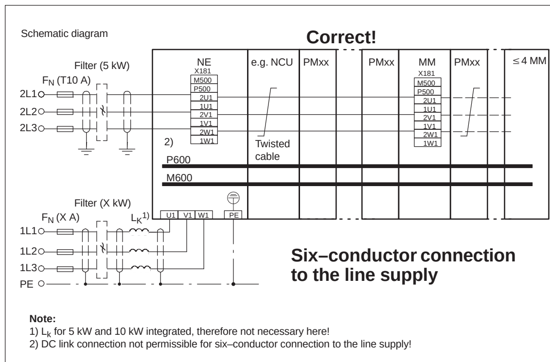
Fig. 8-33 Examples for correct six-conductor connection to the line supply with a maximum of four monitoring modules connected to a line infed module (NE module)
