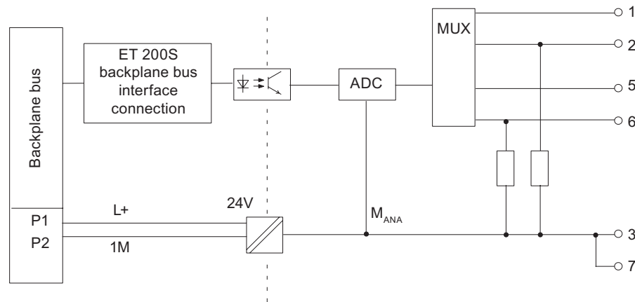
Figure 4-17 Block diagram of the 2AI TC Standard
