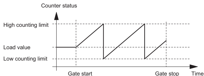
Figure 3-2 Count Continuously with Gate Function
