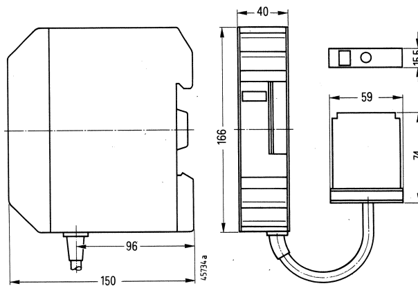
Fig. 22 500 Programmer interface module and 330 test module
