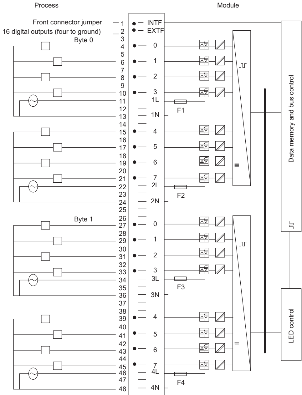
Figure 4-16 Connection and circuit diagram for SM 422; DO 16 x AC 120/230 V/2 A
