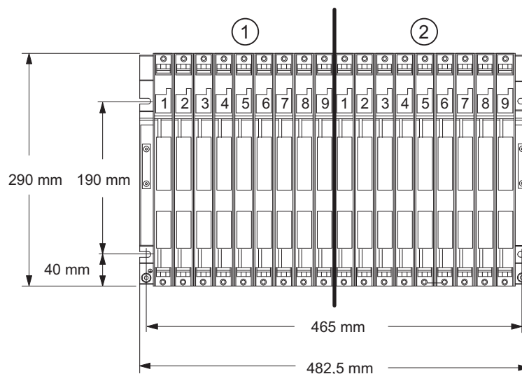
Figure 2-3 Rack dimensions
