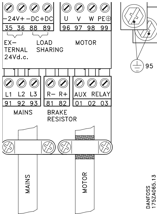
Bookstyle 0.75 - 7.5 kW
