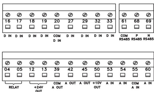
DANFOSS 175HA379.10
