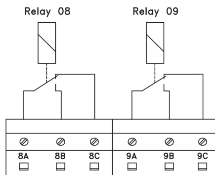
DANFOSS 175HA442.11
