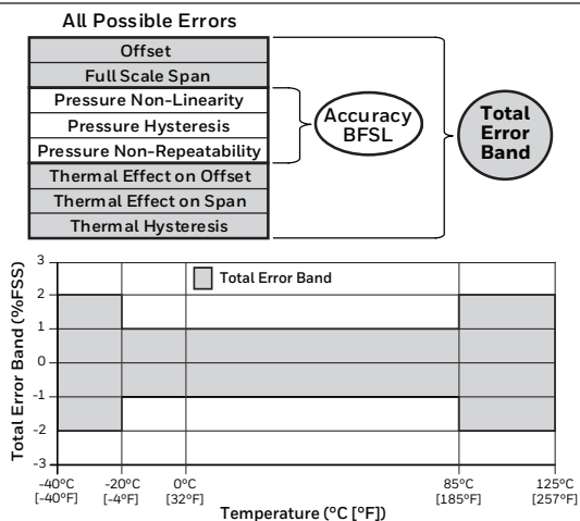
Figure 1. TEB Definition and Temperature Performance
