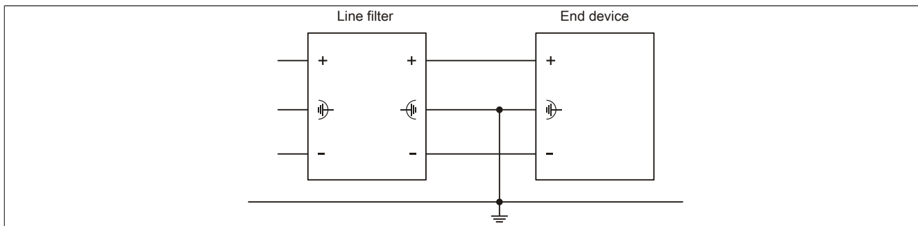
Figure 131: Connection example
