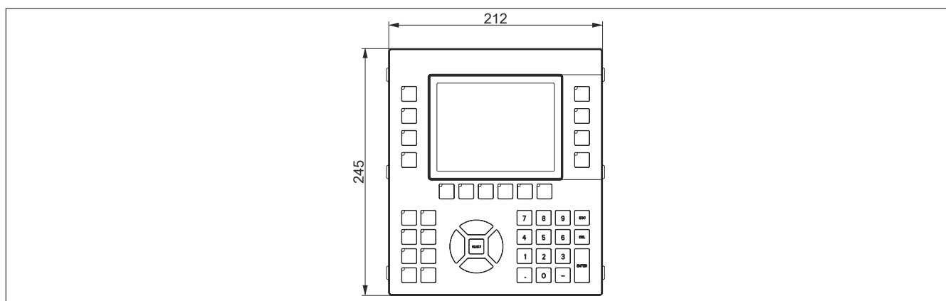
Figure 44: 5AP1151.0573-000 - Dimensions
