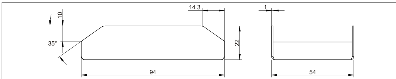
Figure 129: 5AC804.MFLT-00 - Dimensions
