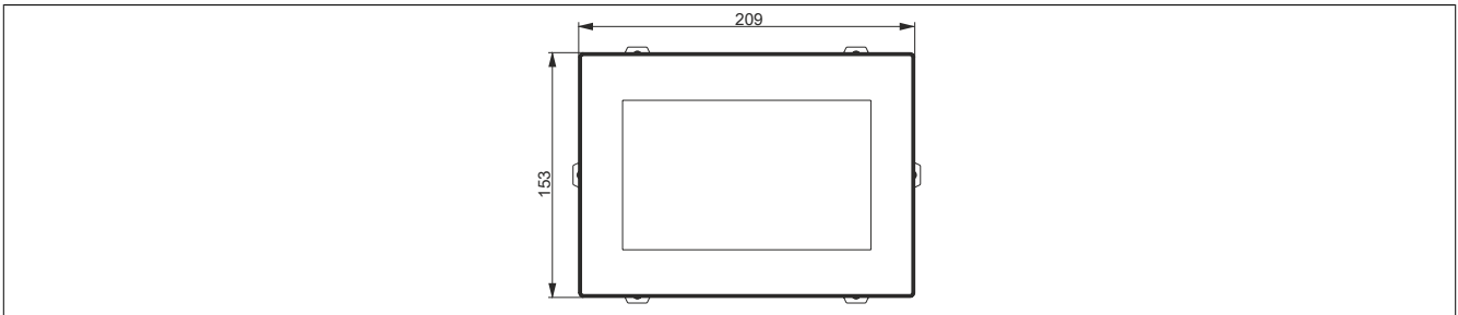
Figure 49: 5AP1130.0702-000 - Dimensions
