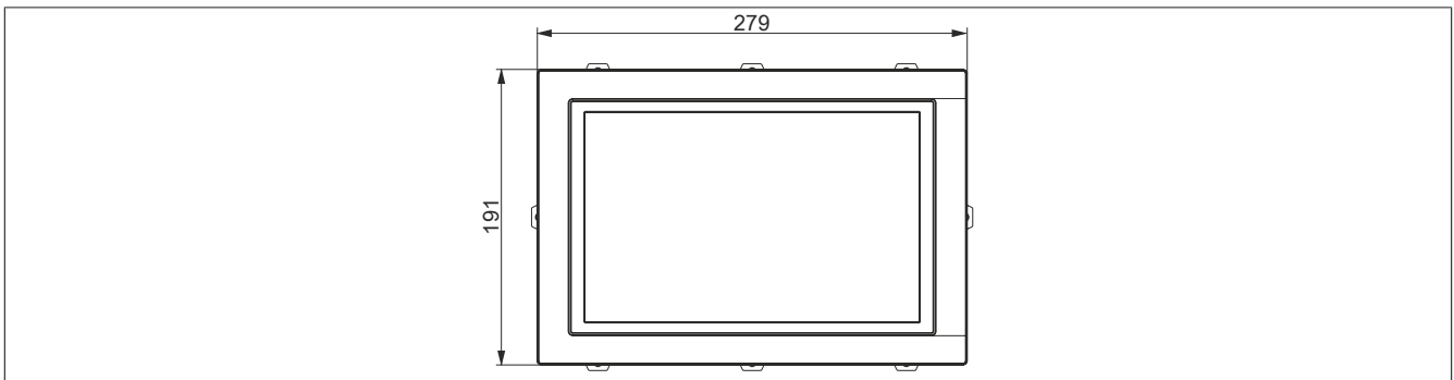
Figure 51: 5AP1120.101E-000 - Dimensions
