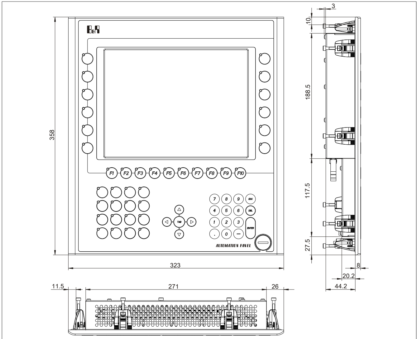
Figure 18: 5AP951.1043-01 - Dimensions
