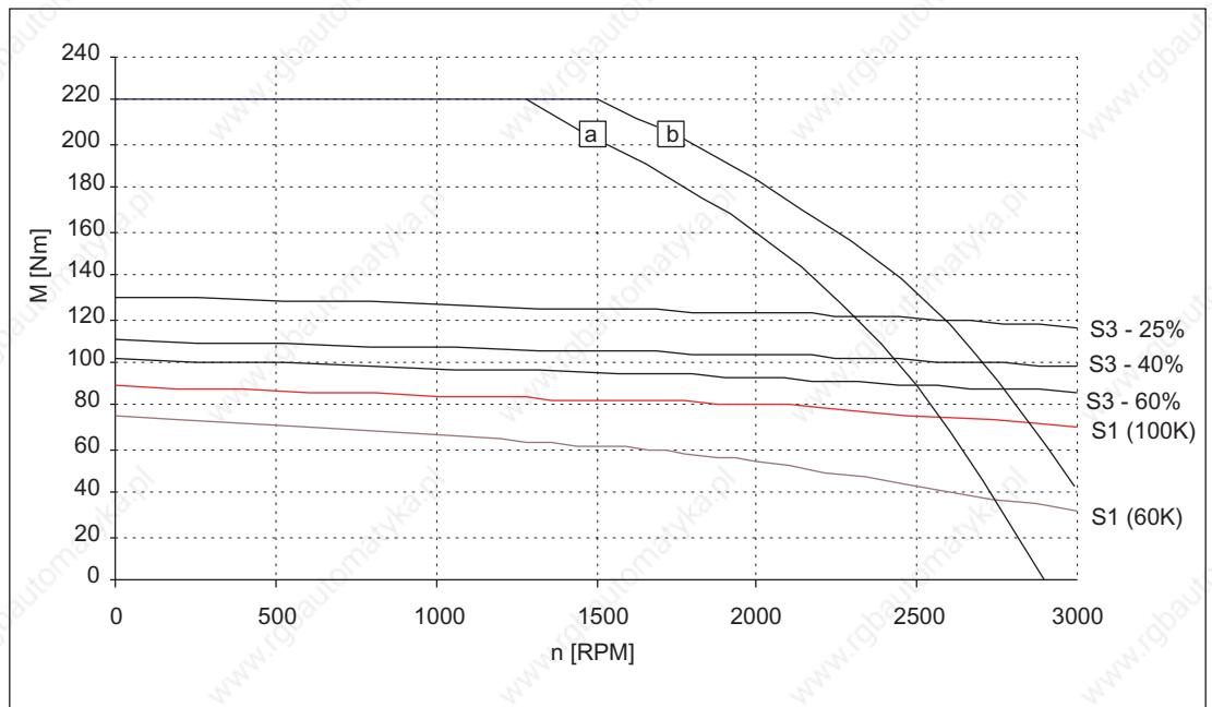
Figure 3-64 Speed-torque diagram 1FT6108-8SC7
