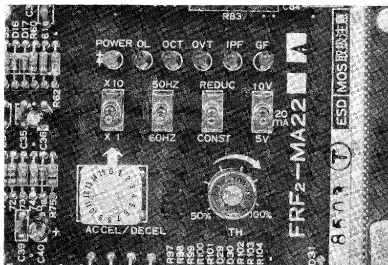
Fig. 15.2.4 Setting Switches
