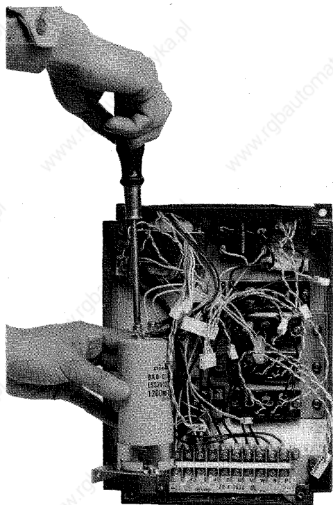
Fig. 15.3.4 Removing Wiring
