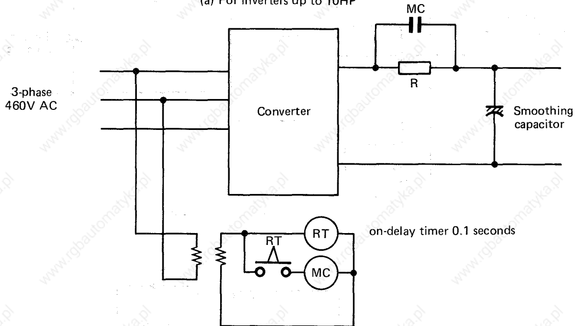
(b) For inverters 20HP throu. 75HP
