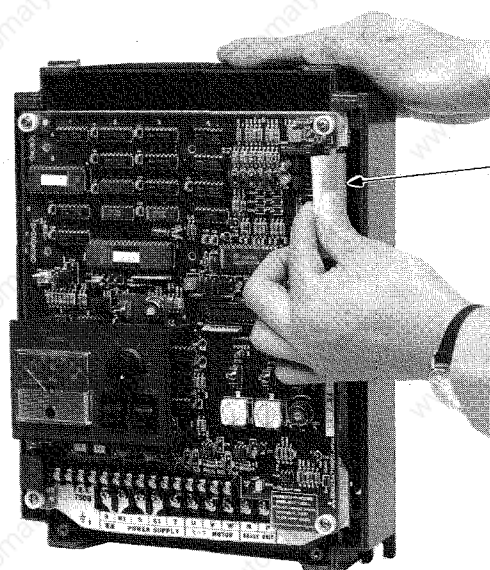
Fig. 15.2.5 Push and Bend The Flat Cable
