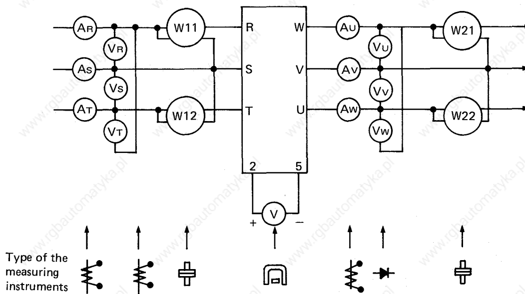
Fig. 14.1 Measuring Points and Instruments
