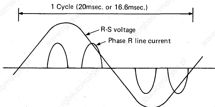
Fig. 10.1 Input Current Waveform of Inverter
