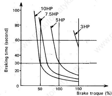
BU-7.5K Short time rating (200V series)
