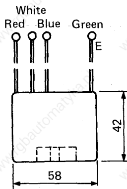
Fig. 11.5 Dimensions of Radio Interference Filter
