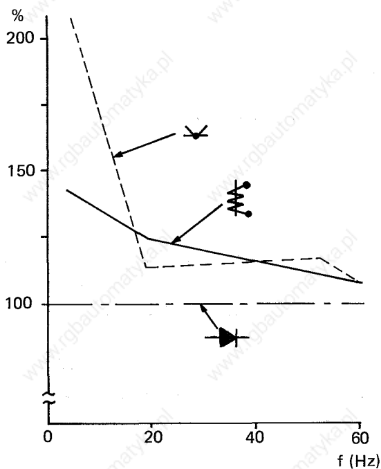
Fig. 14.2 Difference of Indicated Value with Various Measuring Instruments
