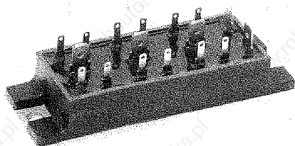
Fig. 6.5.3 Outlook of Six Transistors Packed Type Module
