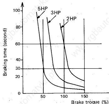
BU-3700 Short time rating (200V series)
