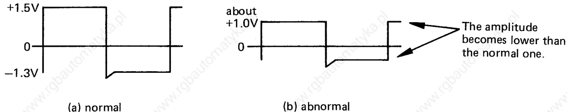
Fig. 6.5.6 B-E Waveform of Power Transistor
