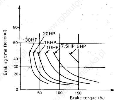
BU-15K Short time rating (200V series)
