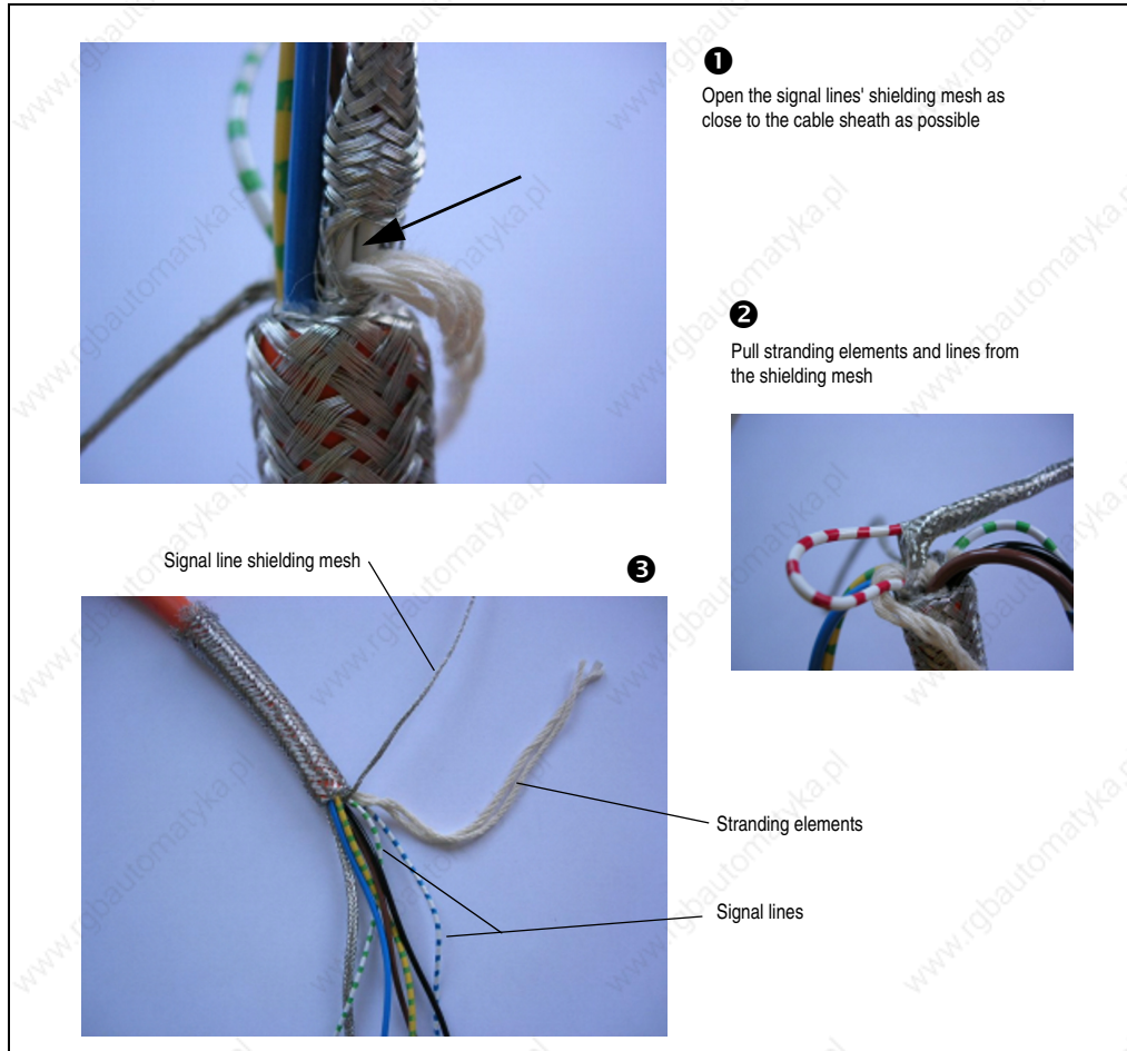
Figure 21: Pulling out the separately shielded signal lines
