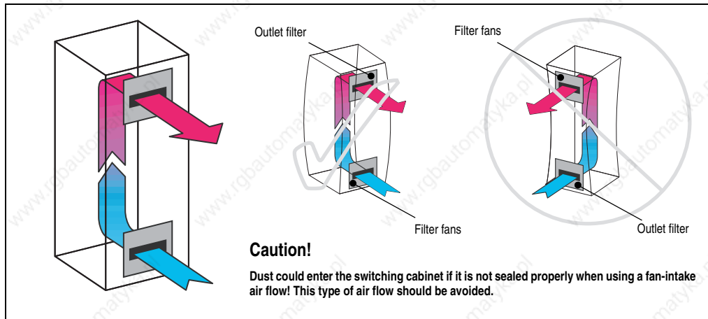
Figure 81: Function diagram of filter fans
