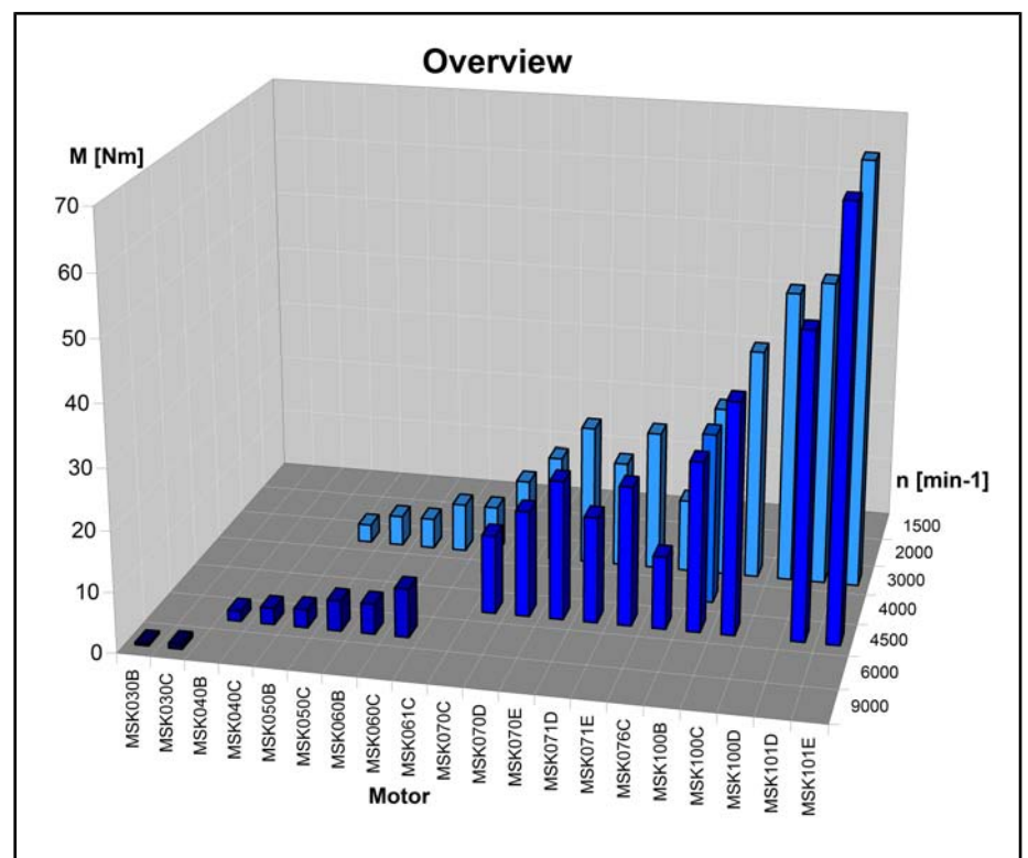
Fig. 1-1: MSK power gradation
