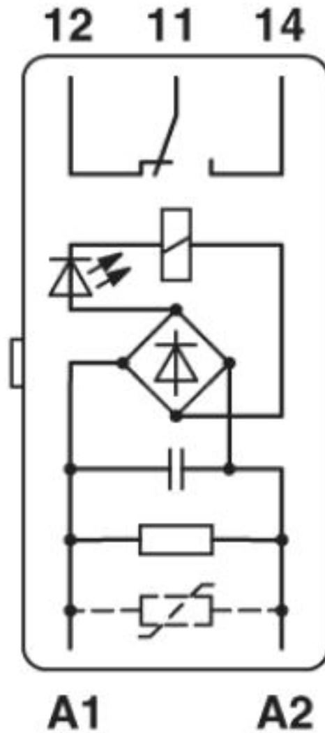
Circuit diagram
