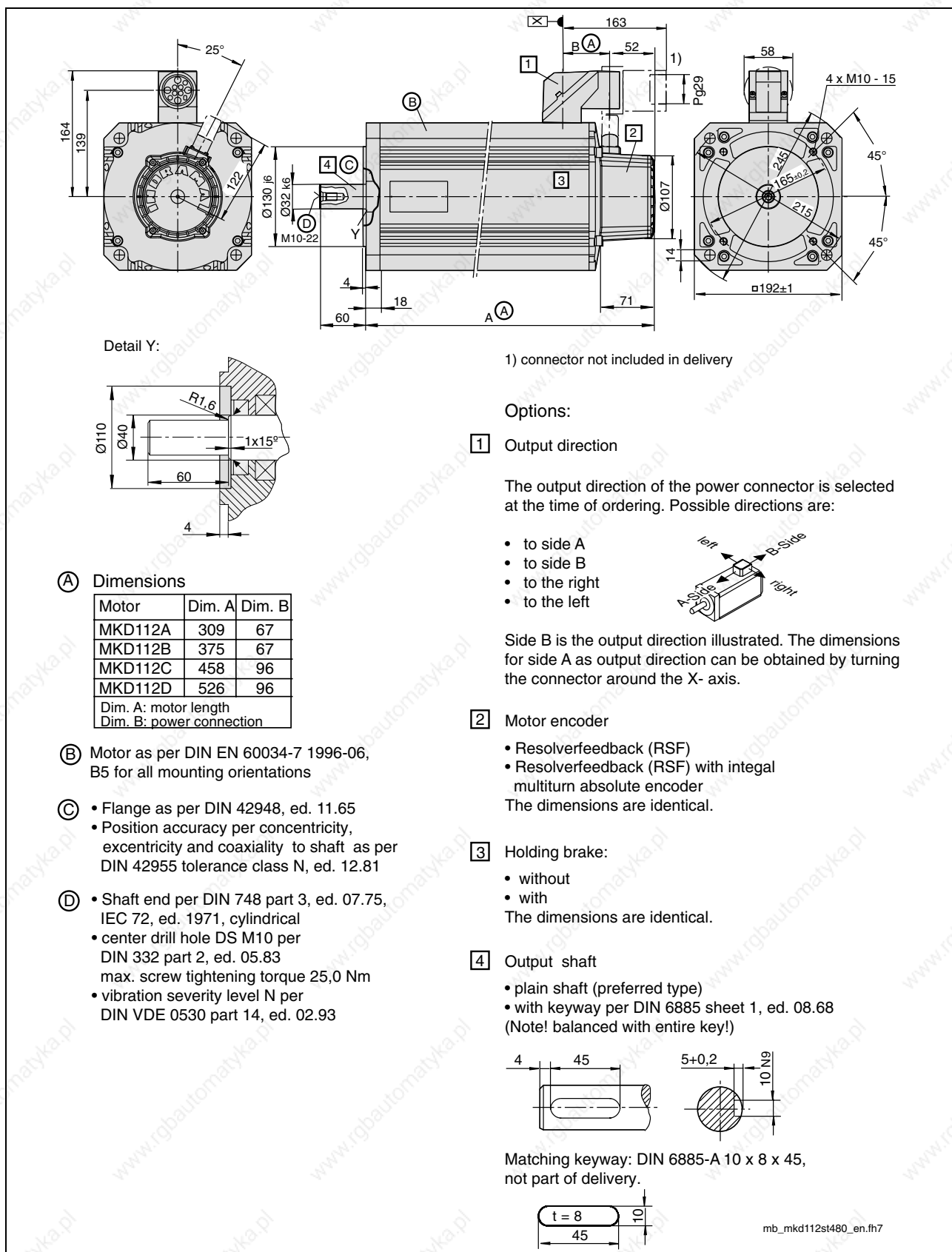
Fig. 10-16: Dimensional data MKD112A, MKD112B, MKD112C 1) , MKD112D 1) not applicable to MKD112C-058
