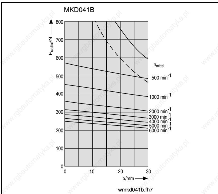
Fig. 7-7: MKD041: Permissible maximum radial force F_{\text{radial\_max}} and permissible radial force F_{\text{radial}}
