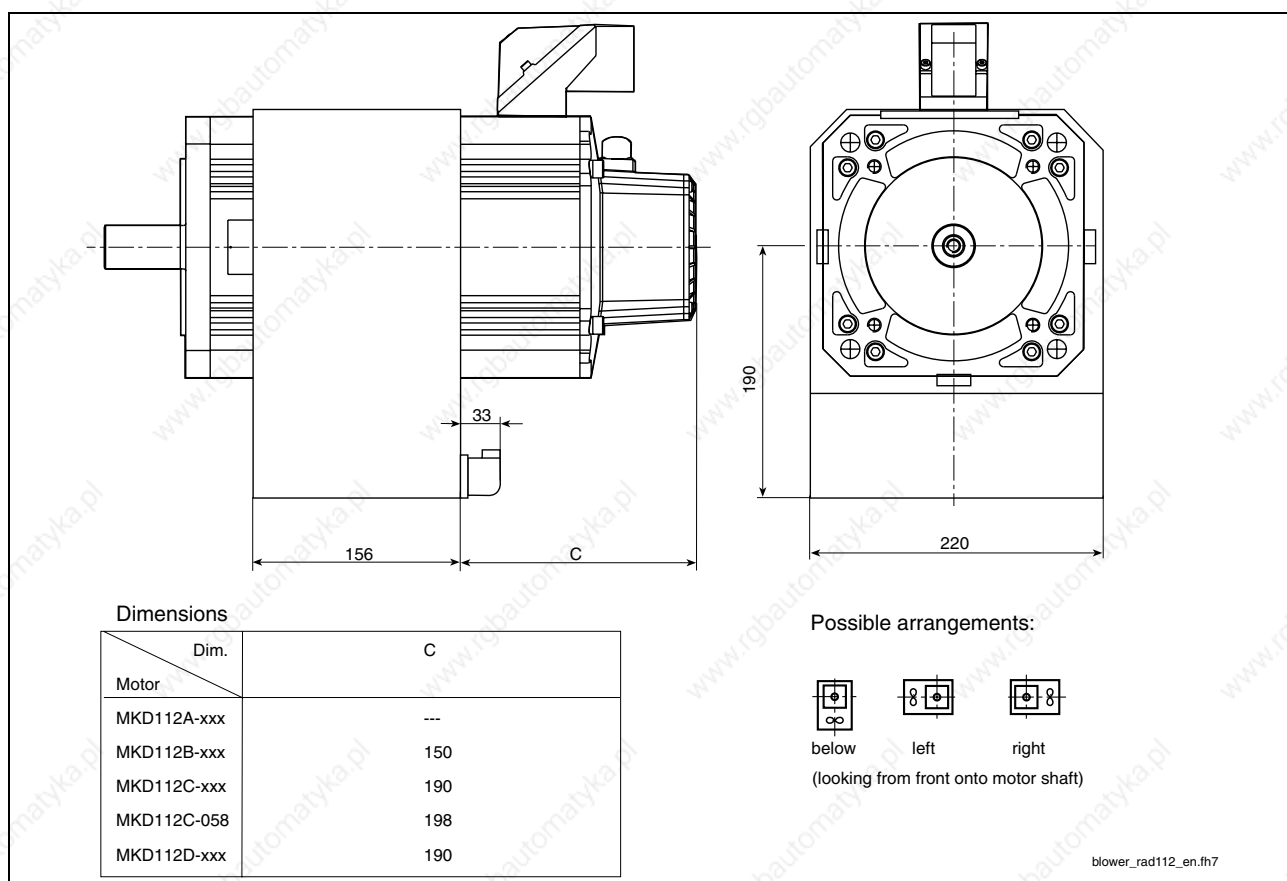
Fig. 10-19: Dimensional data MKD112 with radial blower
