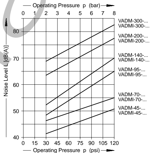
Noise level as a function of operating pressure
