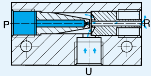
Type VAD-1/4
