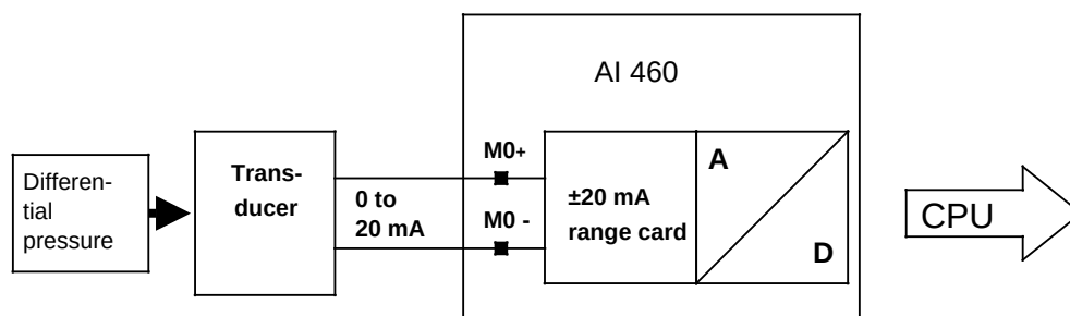
Figure 10-31. Function of the 460 Analog Input Module
