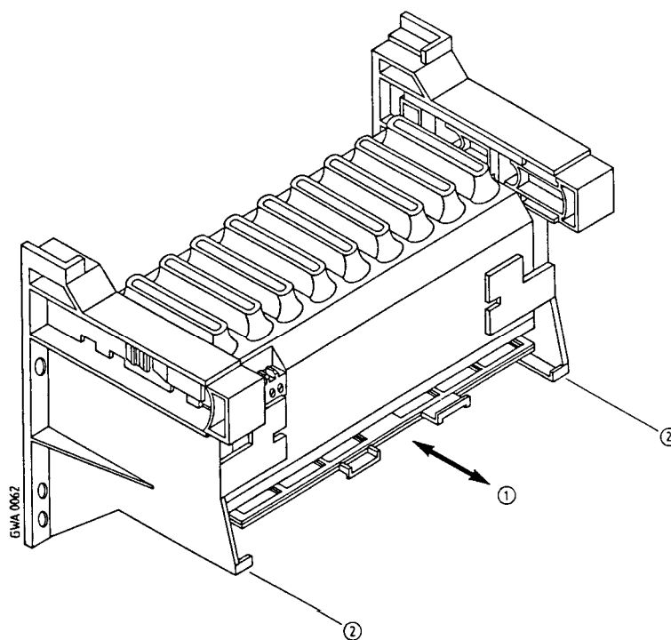
Figure B-2. Changing the Fan Filter
