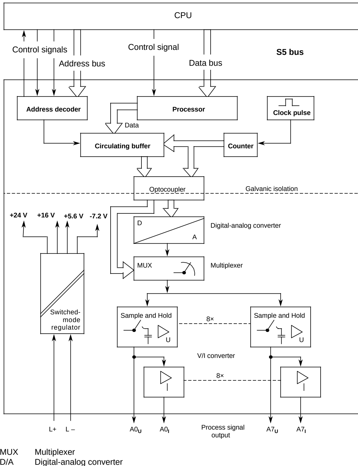
Figure 10-25. Block Diagram with Signal Interchange between CPU and a 470 Analog Output Module
