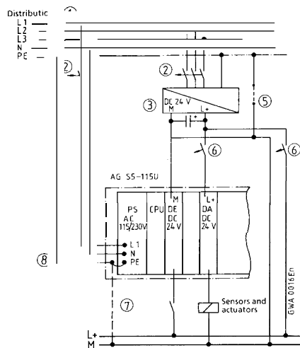
Installation with 115 V AC/230 V AC for the PLC and 24 V DC Power Supply for Sensors and Actuators
