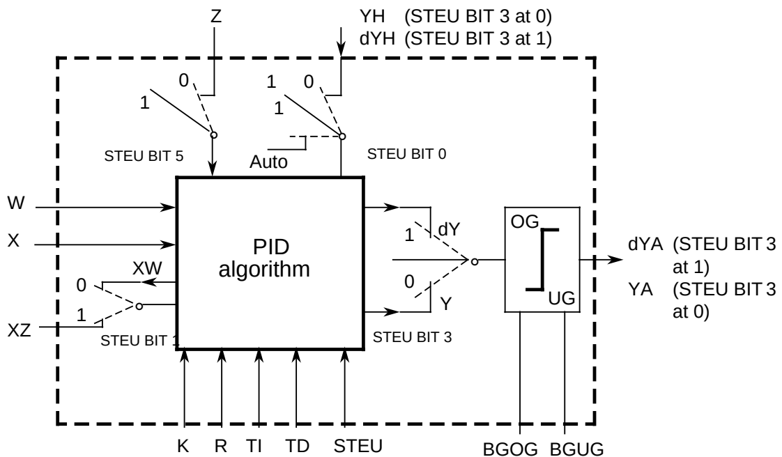
Figure 11-3. Block Diagram of the PID Controller
