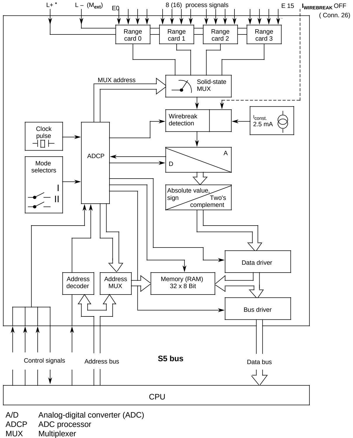
Figure 10-11. Block Diagram with Signal Interchange between a 465 Non-Isolated Analog Input Module and the CPU
