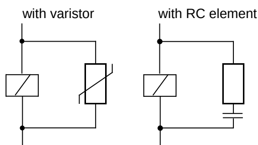
Figure 3-31. Connecting Coils
