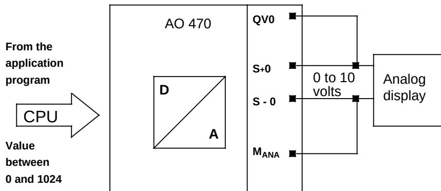
Figure 10-33. Function of the 470 Analog Output Module
