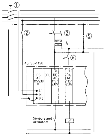
Installation with 115 V AC/230 V AC for PLC, Sensors and Actuators
