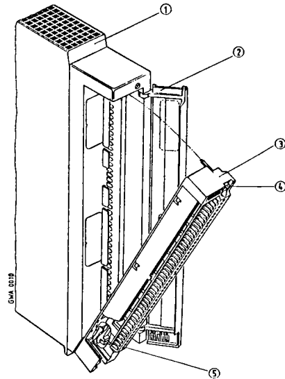
Figure 3-26. Installing the Front Connector
