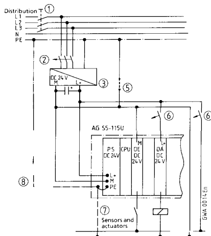
Installation with 24 V DC Power Supply for PLC, Sensors and Actuators
