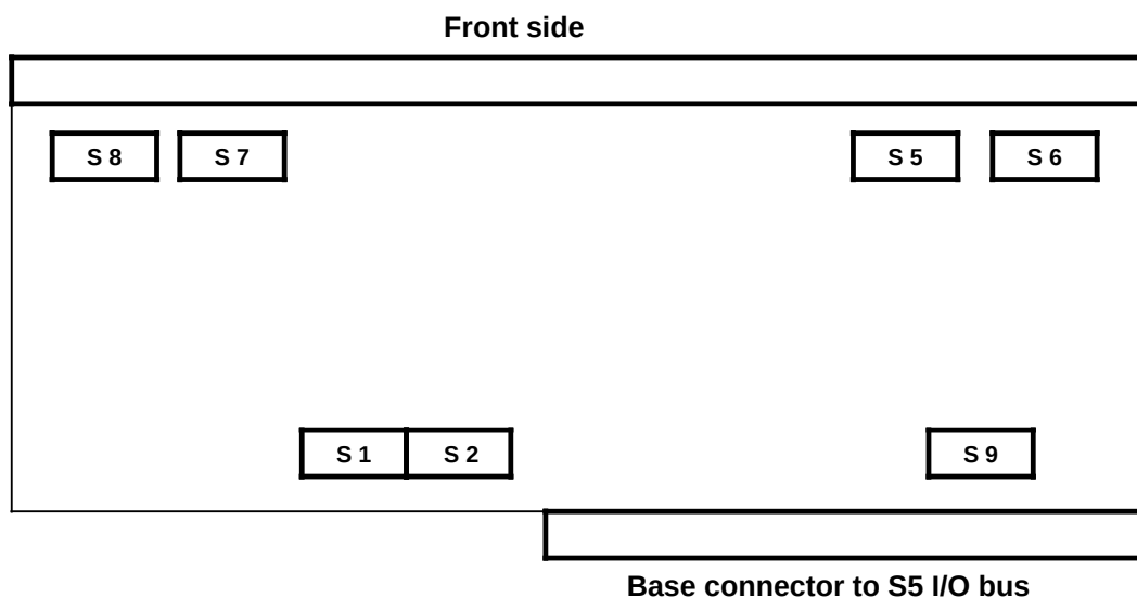
Figure 10-21. Locations of the Mode Selectors on the 466-3LA11 Analog Input Module
