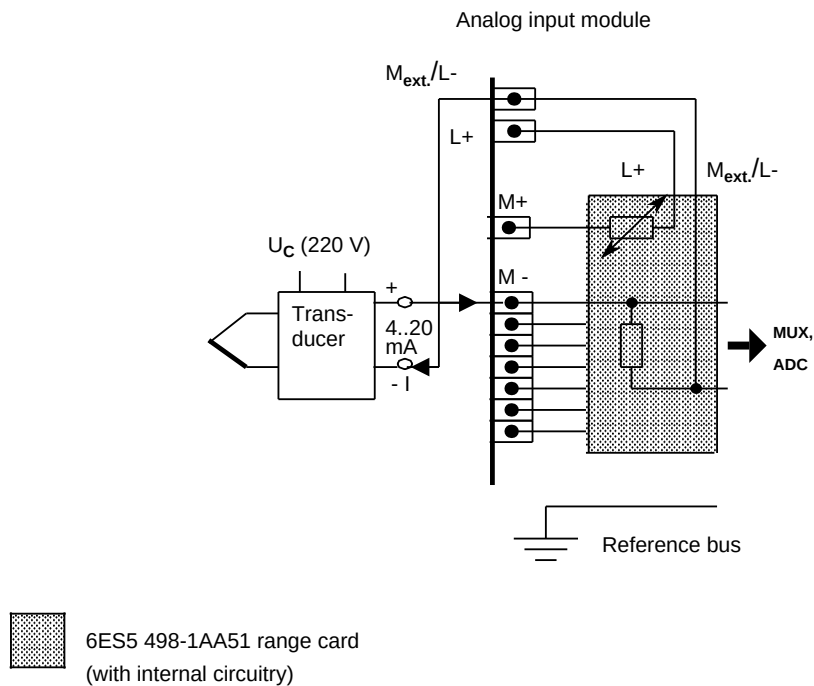
Figure 10-9. Connecting Transducers (Four-Wire Transducer to a Two-Wire Range Card)
