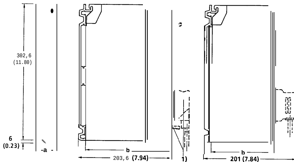
Figure 3-16. Dimension Drawings of Mounting Racks
