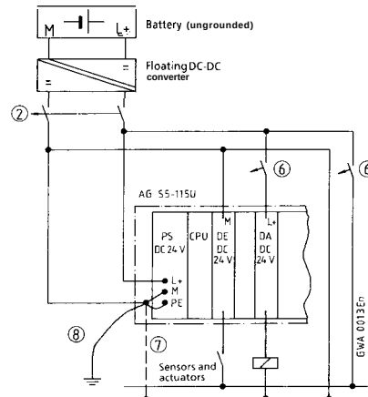
Installation with 24 V DC Power Supply from Nongrounded Battery for PLC, Sensors and Actuators. PC is grounded.
