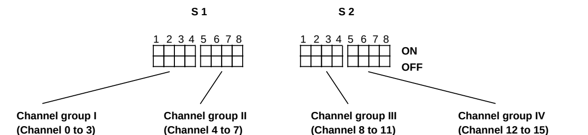
Figure 10-22. Assignment of Switches S 1/S 2 to Channel Group
