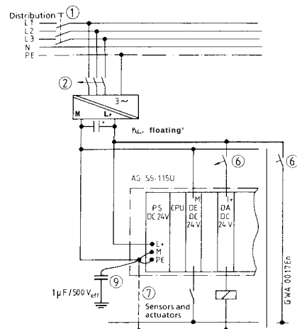
Installation with 24 V DC Power Supply for PLC, Sensors, and Actuators (Nongrounded). For floating operation, the 24V DC supply voltage must be safety extra-low voltage in accordance with VDE O 100/5.73 § 8c or comparable standard.
