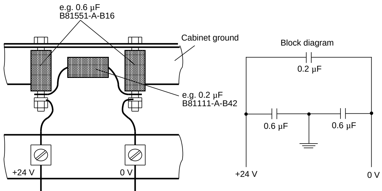
Figure 3-30. Arrangement of Suppression Capacitors
