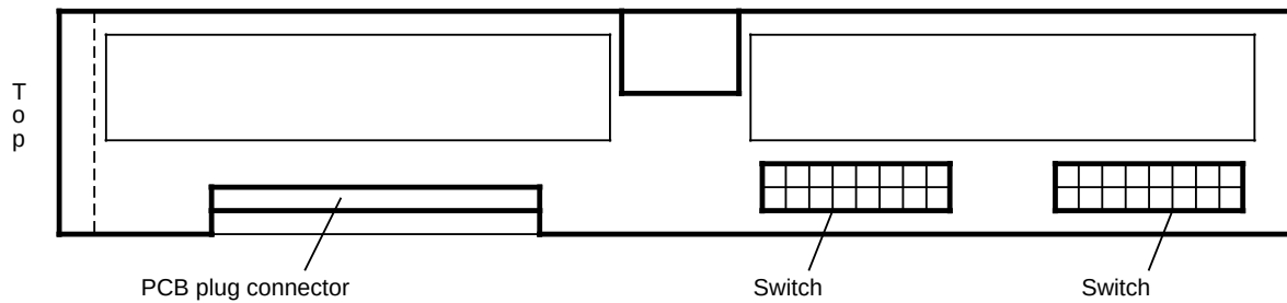
Figure 10-15. Position of the Function Select Switches of the 465-7LA12 Analog Input Module (Rear of the Module)
