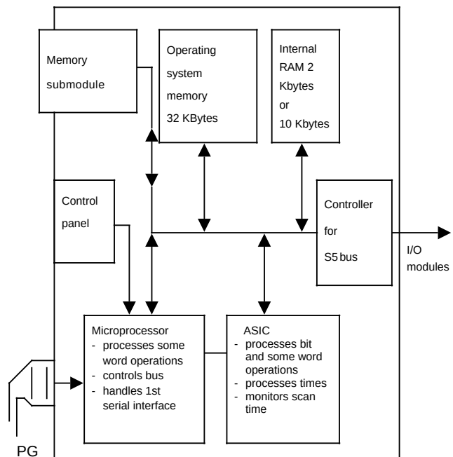
Figure 2-4. Schematic Representation of CPU 941 and CPU 942
