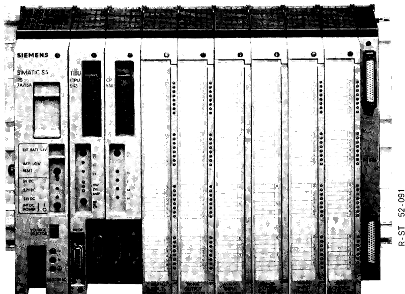
Figure 3-1. Central Controller (Example)
