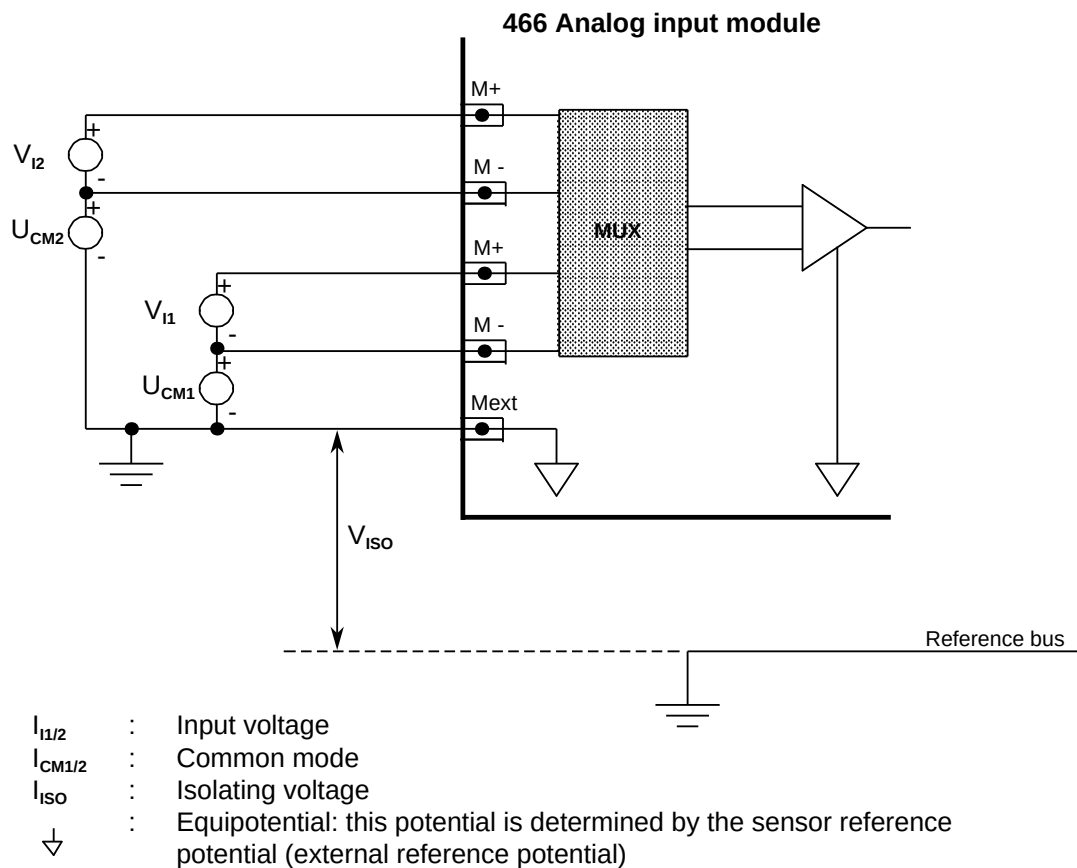
Figure 10-20. Connecting Transducers to the 466 Analog Input Module (Differential Measurement)
