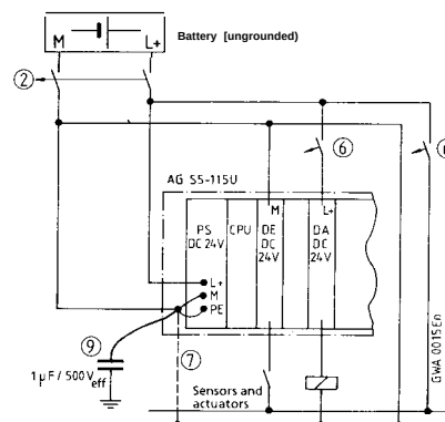
Installation with 24 V DC Power Supply from Nongrounded Battery for PLC, Sensors and Actuators. PC is not grounded.
