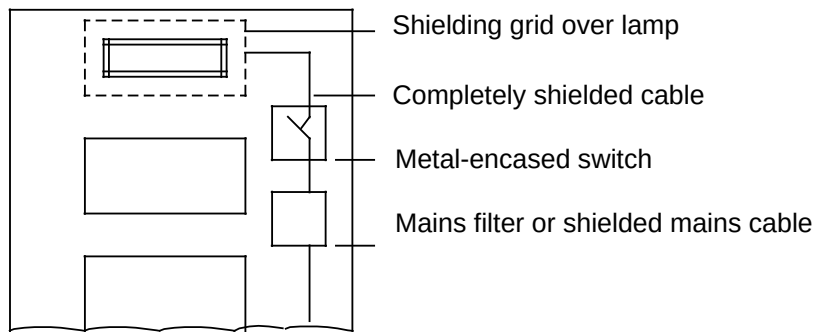
Figure 3-32. Measures for Suppressing Noise from Fluorescent Lamps in the Cabinet
