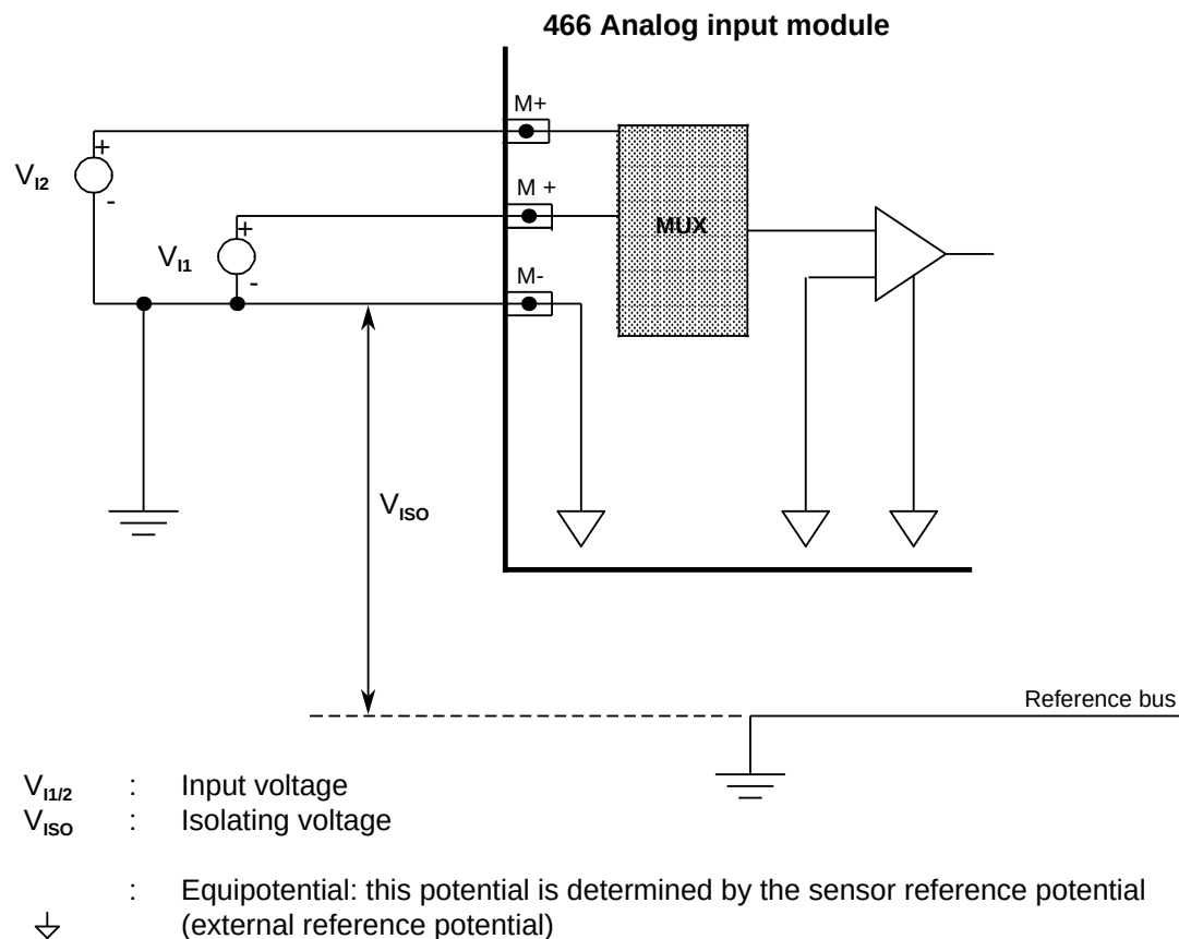
Figure 10-18. Connecting Transducers to the 466 Analog Input Module (Common-Reference Measurement)
