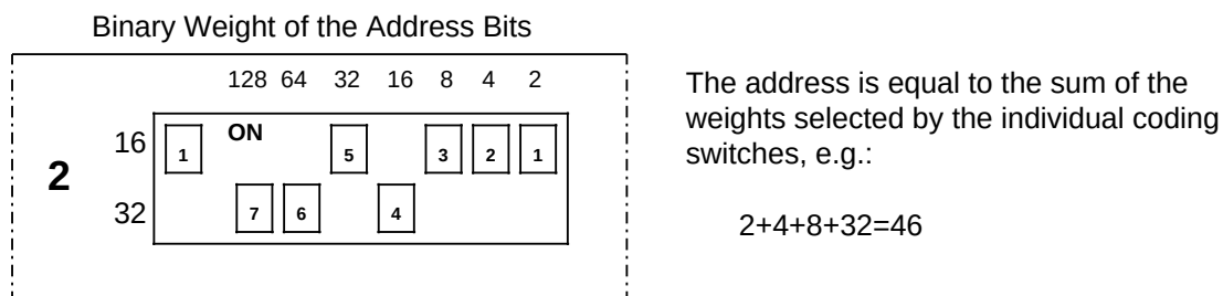
Figure 6-5. Setting a DIP Switch
