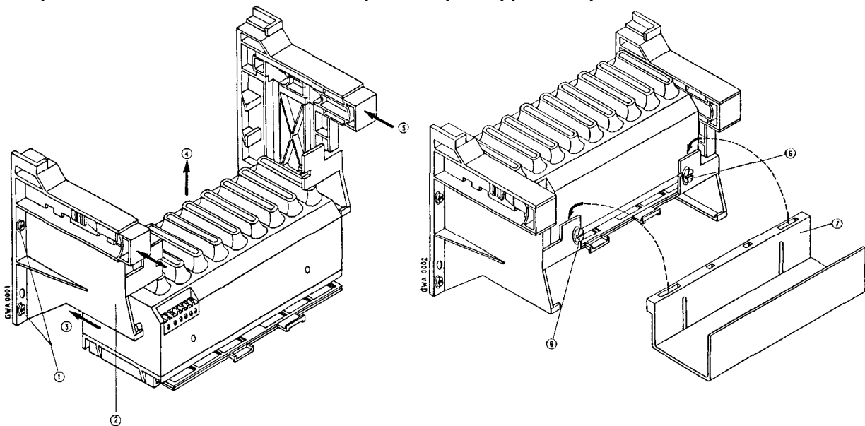
Figure 3-15. Installing the Fan Subassembly
