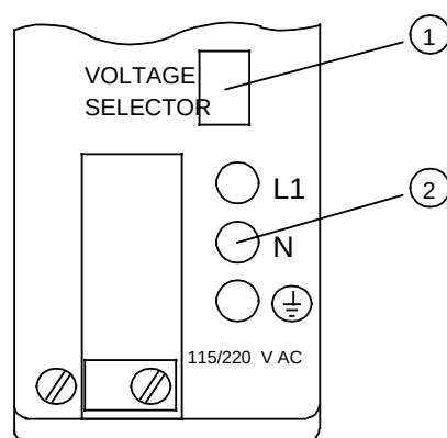
Figure 3-23. Power Supply Module PS 951
