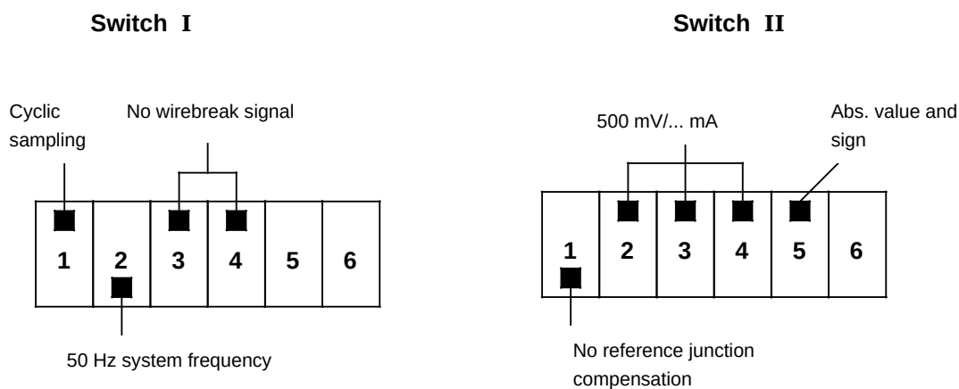
Figure 10-32. Setting Mode Selectors I and II
