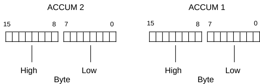
Figure 8-1. Accumulator Structure
