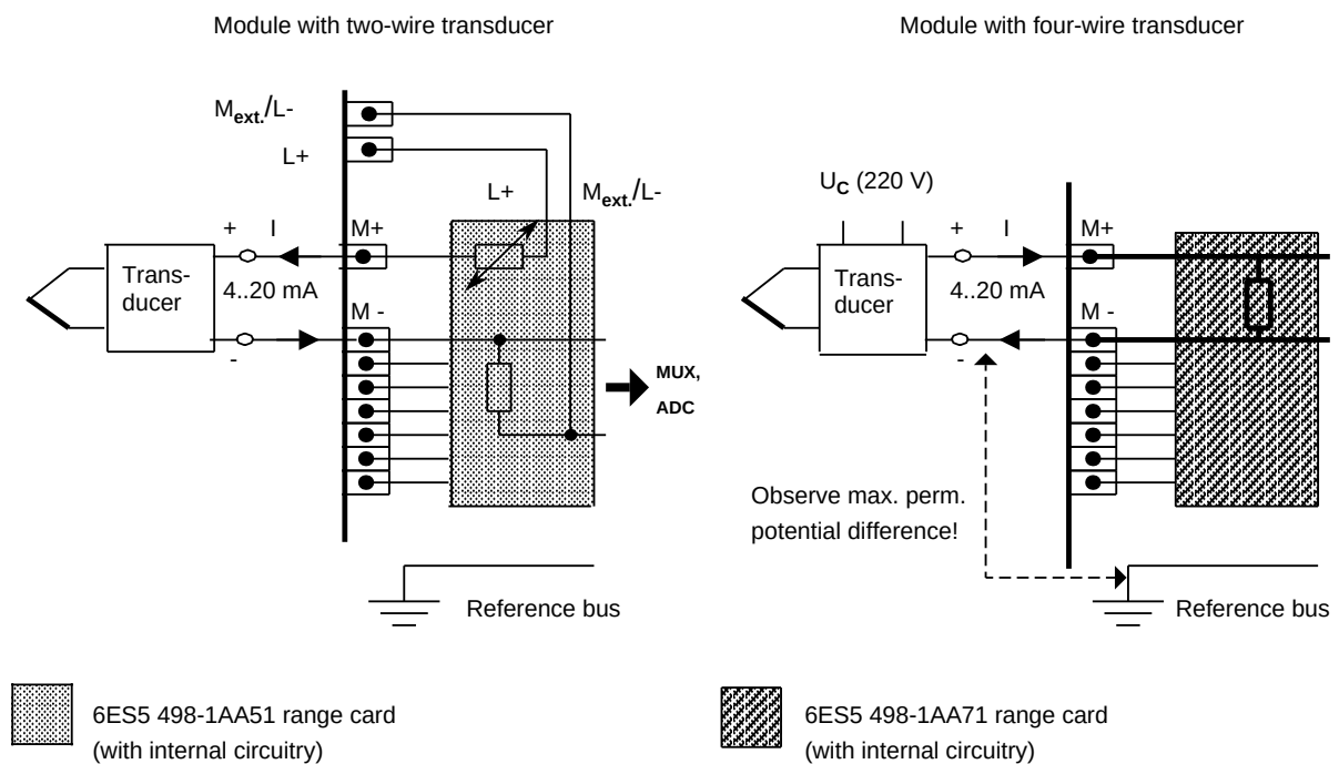
Figure 10-8. Connecting Transducers
