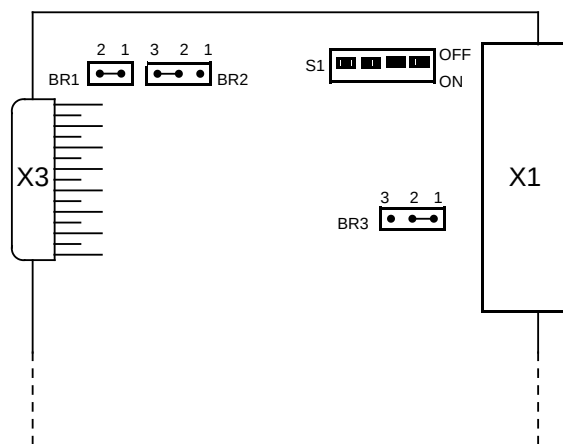
Figure 3-22. Jumper Settings on the IM 314
