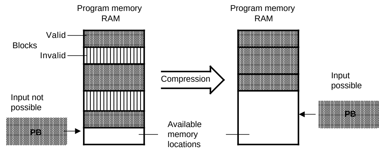
Figure 7-10. Compression Process
