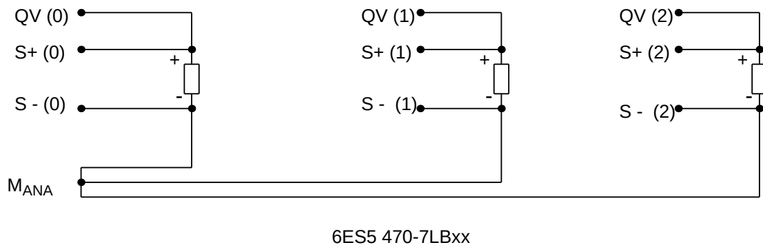
Figure 10-27. Connecting Loads to Current and Voltage Outputs
