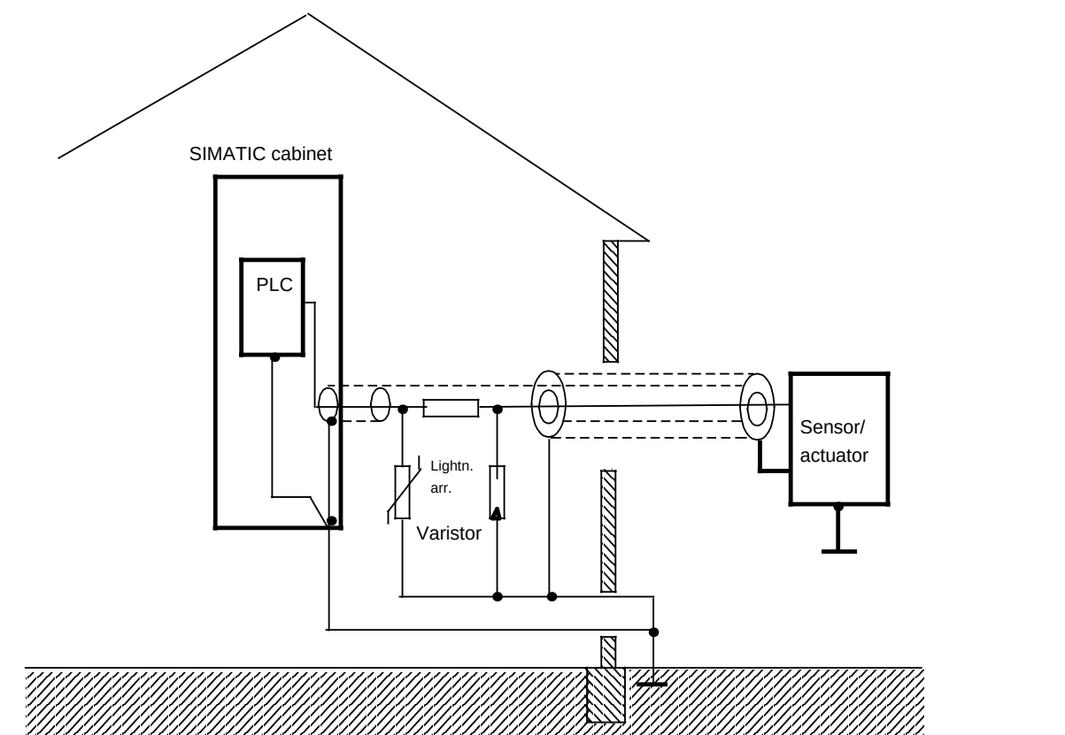
Figure 3-33. Arrangement of Lightning Protection Elements
