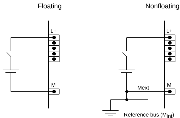
Figure 3-24. Connection to Floating and Nonfloating Modules
