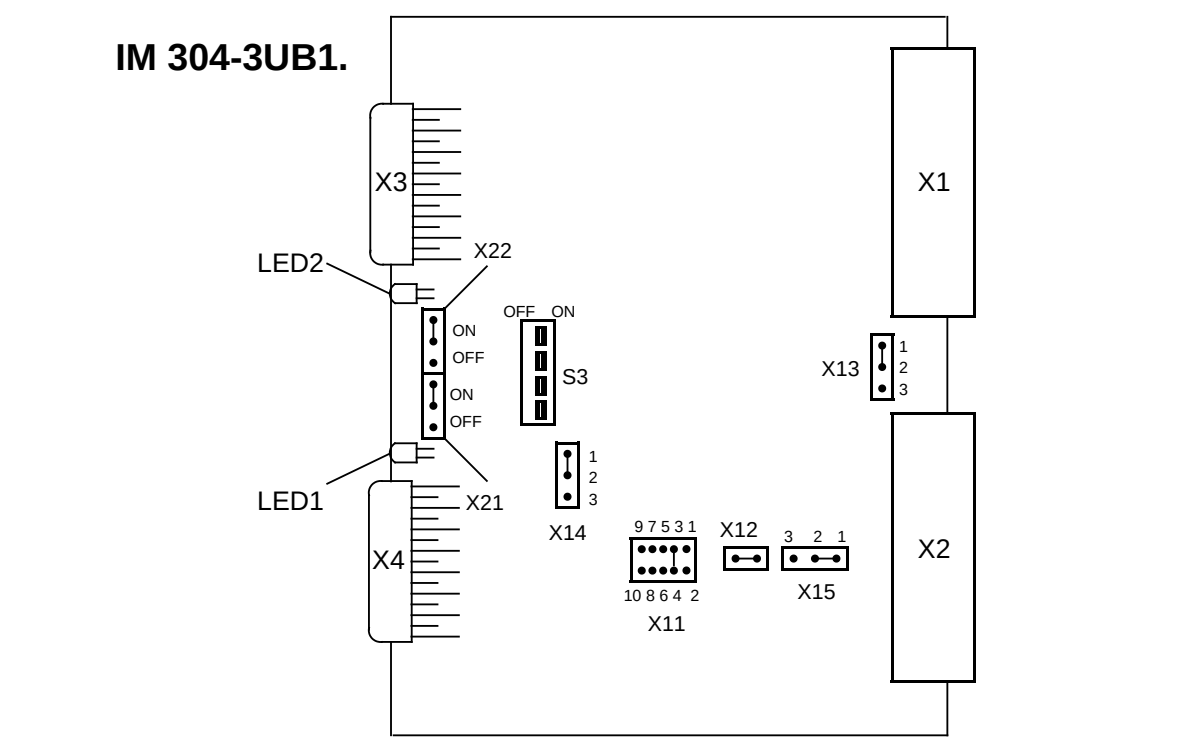
Figure 3-21. Switch and Jumper Settings on the IM 304-3UB1. for Distributed Connection
