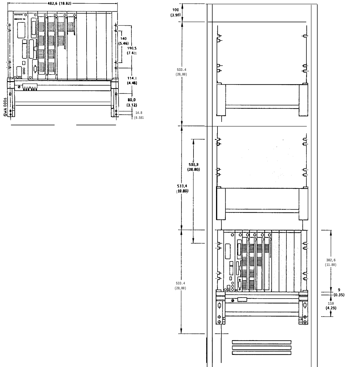
Figure 3-17. Dimensions for Installation in a 19-inch Cabinet
