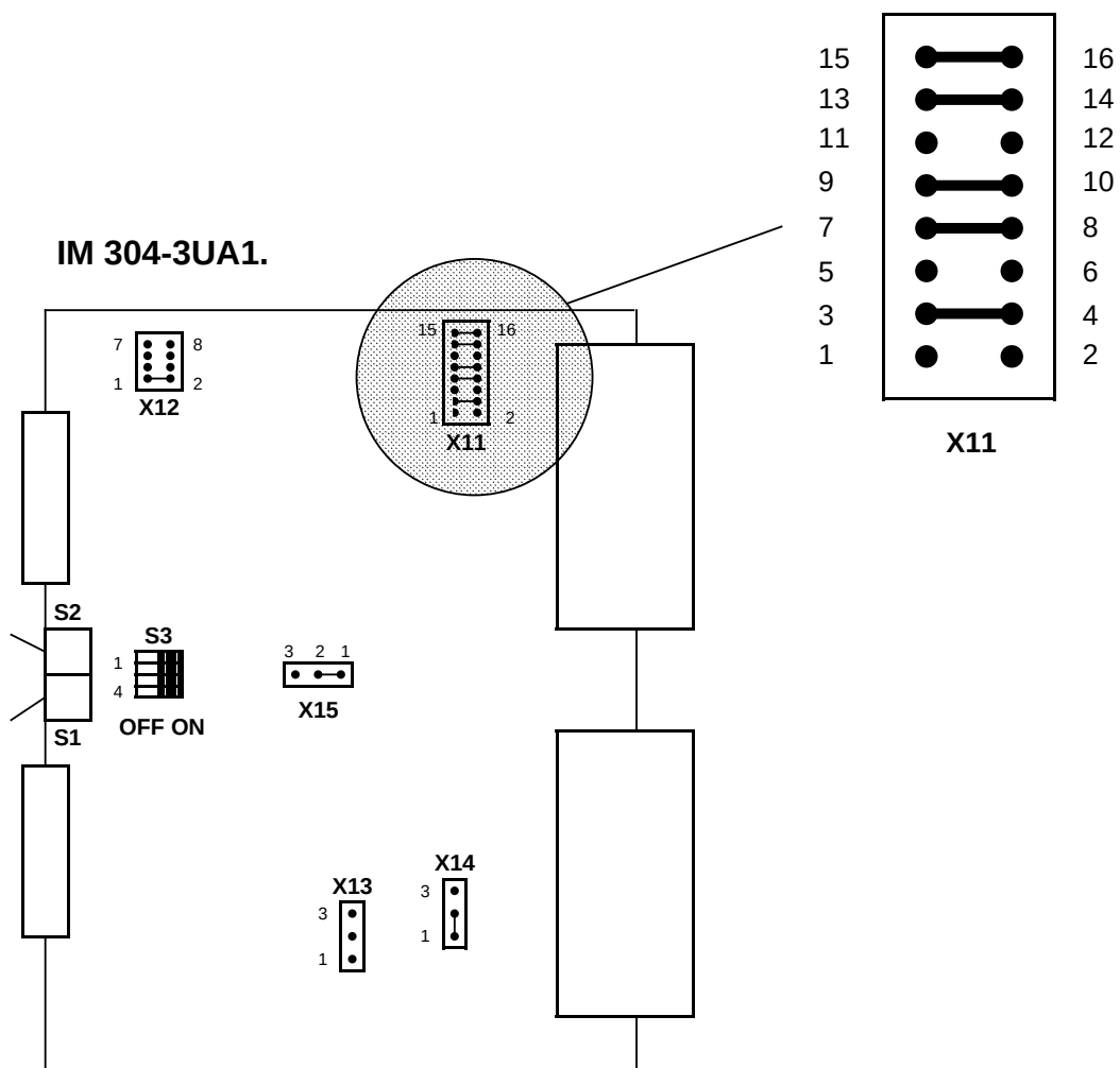
Figure 3-20. Switch and Jumper Settings on the IM 304-3UA1. for Distributed Configurations
