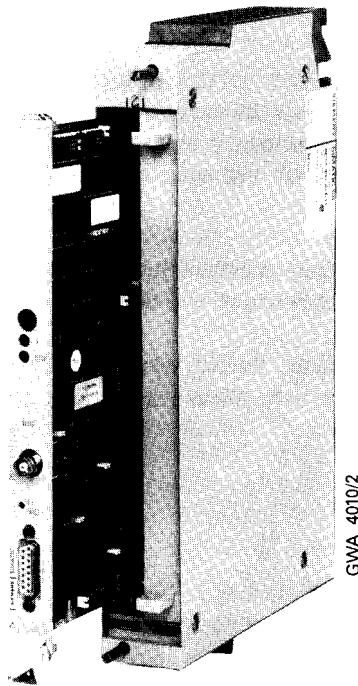
Figure 3-14. Installation of a Printed Circuit Board into an Adapter Casing (6 ES5 491-OLB11)
