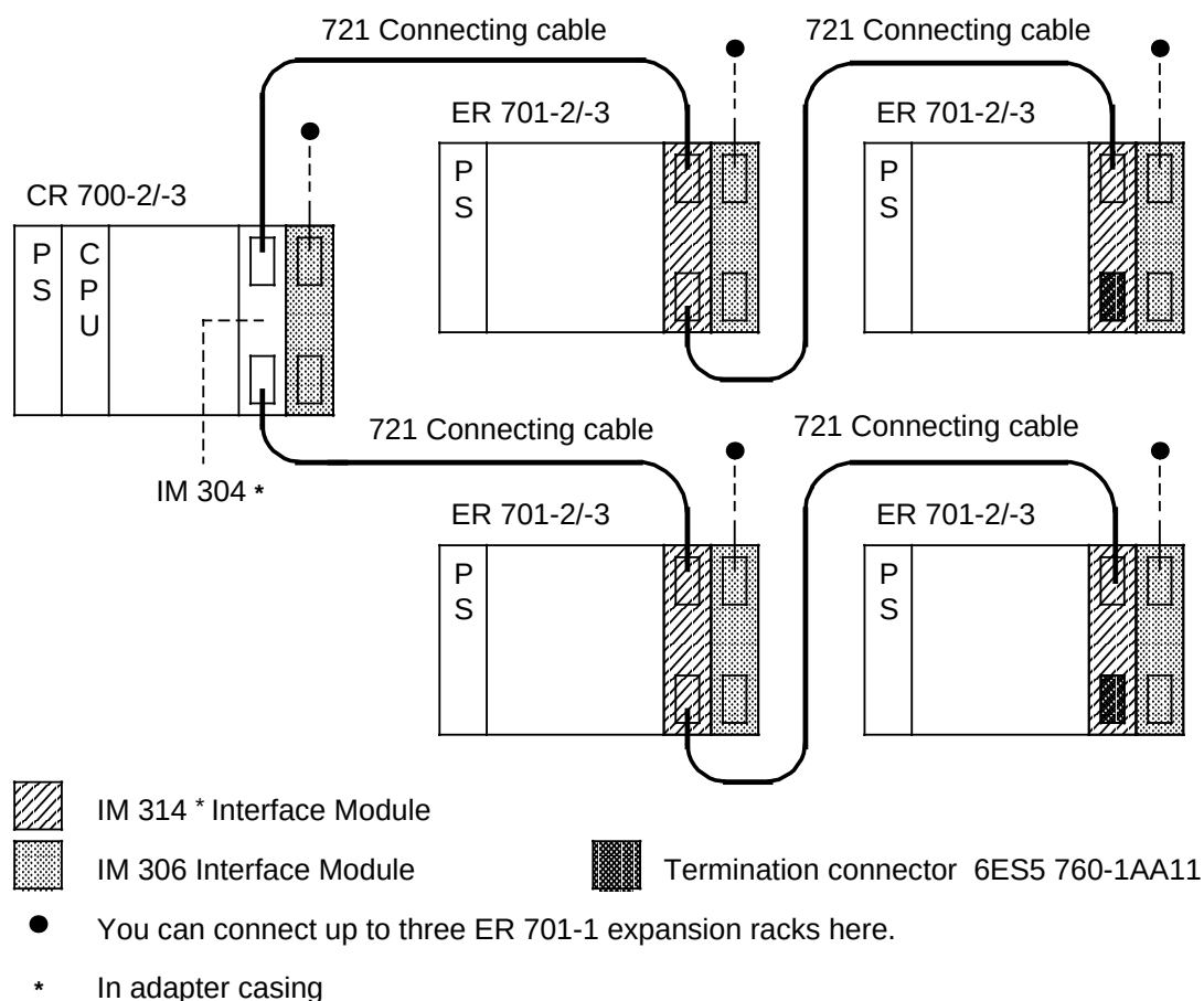
Figure 3- 19. Distributed Configuration with IM 304/IM 314
