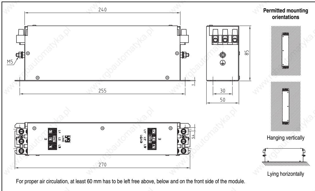
Figure 31: Dimension diagram and installation dimensions for 8B0F0300H000.000-1
